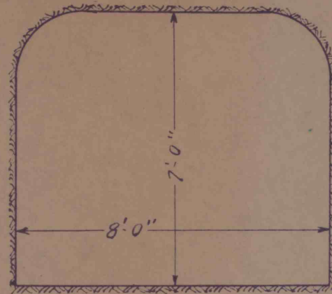
TYPICAL SECTION OF TUNNEL SCALE 1/4" = 1 FT.
