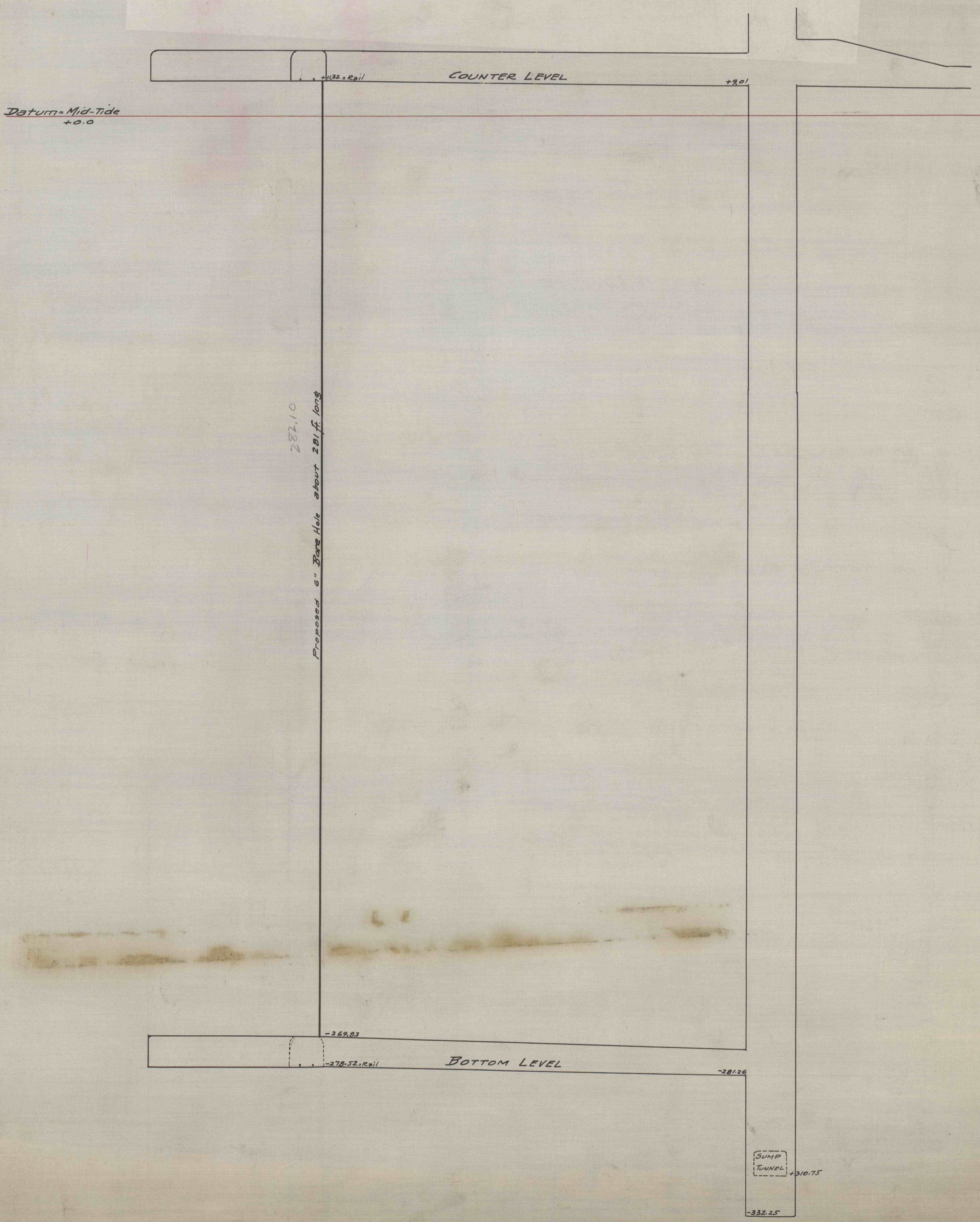
Plan and Profile N o 2 Shaft Counter & Bottom Levels showing location of Proposed 6" Water Hole. Lykens, Pa., May 9 th 1913. Scale 1"=20'
