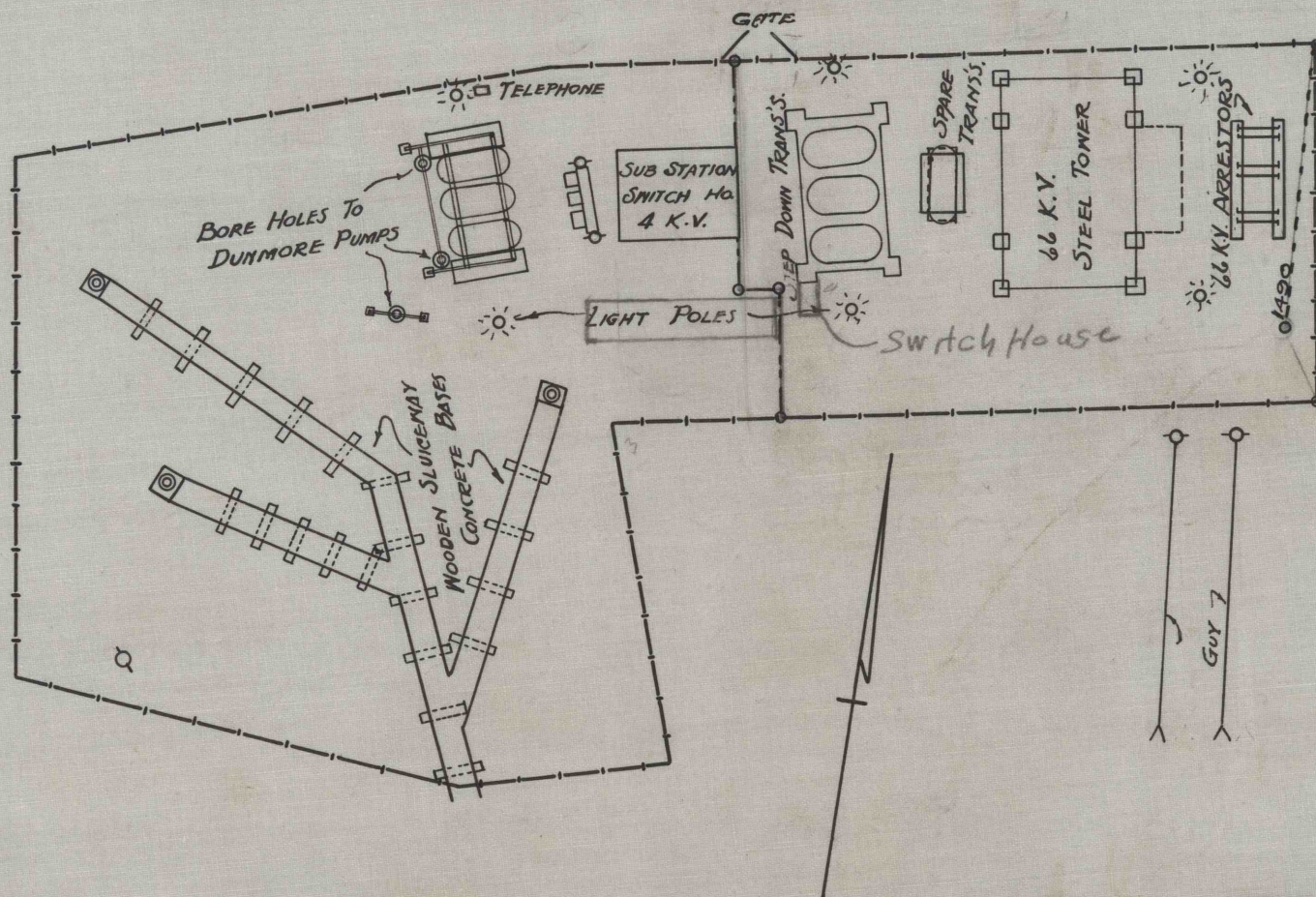
PLAN OF FEEDERDAM SUB STATION AND.
