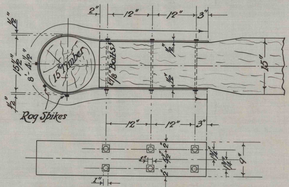
1" Detail of 1/2" Steel Plate for Timber Block
