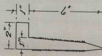
6" Rag Spike for Block Support.
