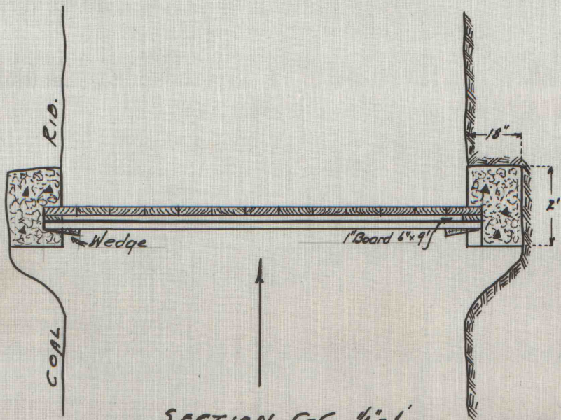
SECTION C-C \frac{1}{2}'' = 1'
