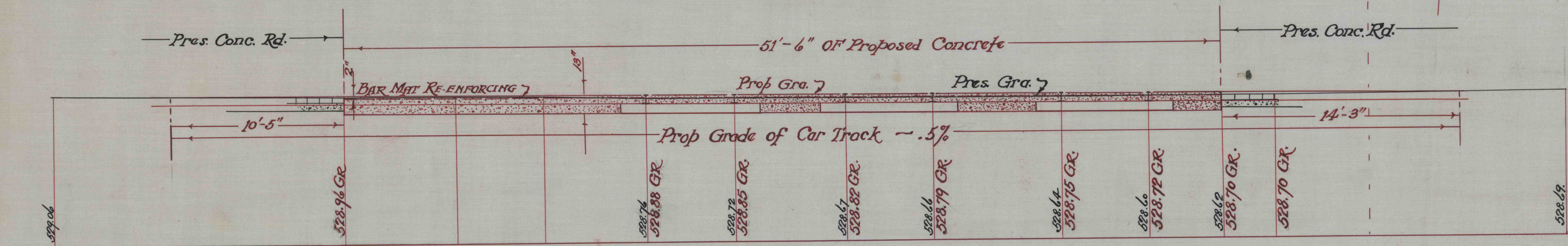
1/4 SECTION B-B' - AT STREET RAILWAY
