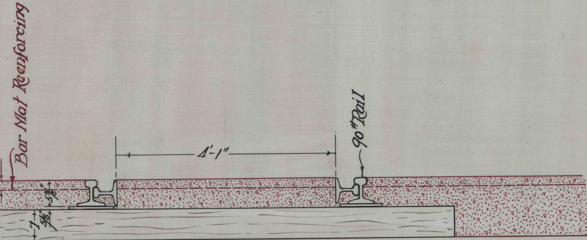
DETAIL SECTION SHOWING PROPOSED RAIL FLANGED WITH RAIL AND PROPOSED BAR MAT REINFORCING OF CONCRETE SCALE 1"=1'
