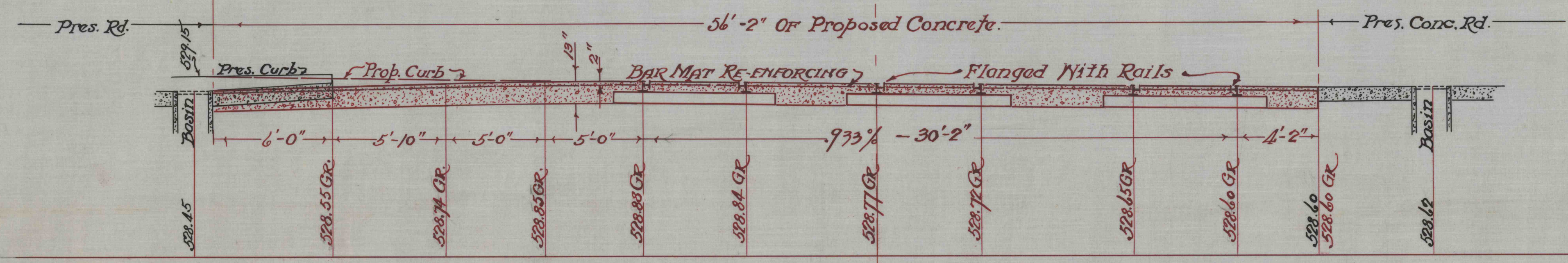
1/4 SECTION A-A' - AT PROPOSED GRADE LINE OF CURB NORTH SIDE
