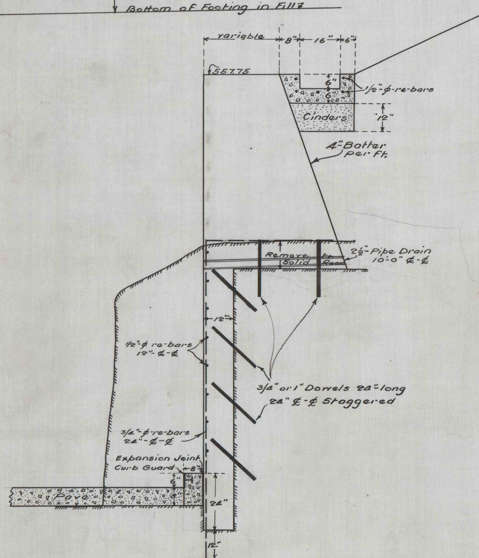
TYPICAL SECTION ON ROCK
