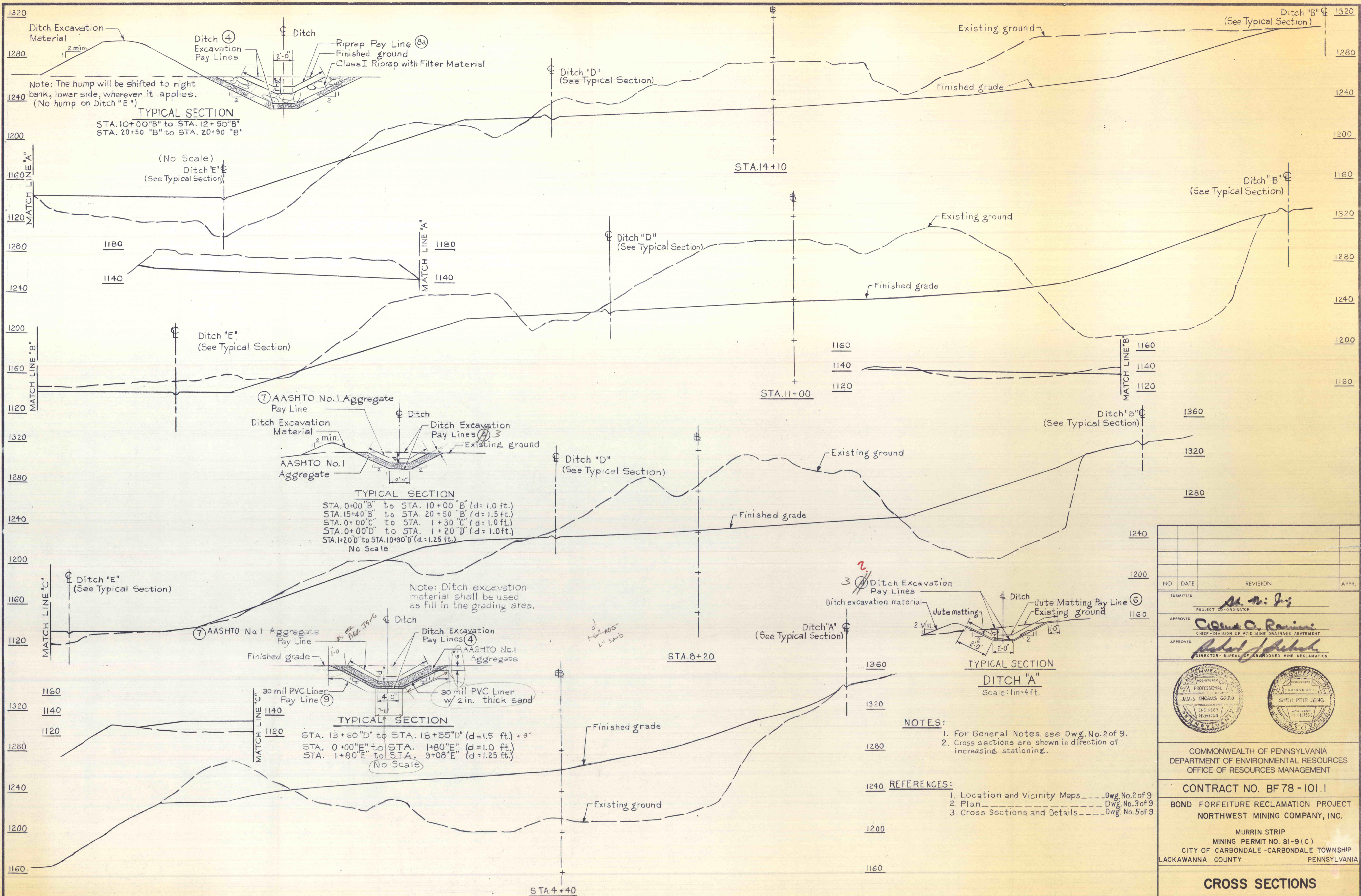
CROSS SECTIONS Scale: 1 in = 40 ft.
