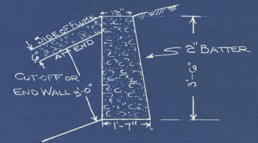
TYPICAL SECTION THROUGH WING WALLS SCALE: 1"=2'
