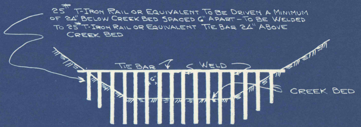
TYPICAL SECTION OF TRASH RACK TO BE INSTALLED 50' FROM END OF EACH SPUR & EAST & WEST BRANCHES - SCALE: 1"=4'
