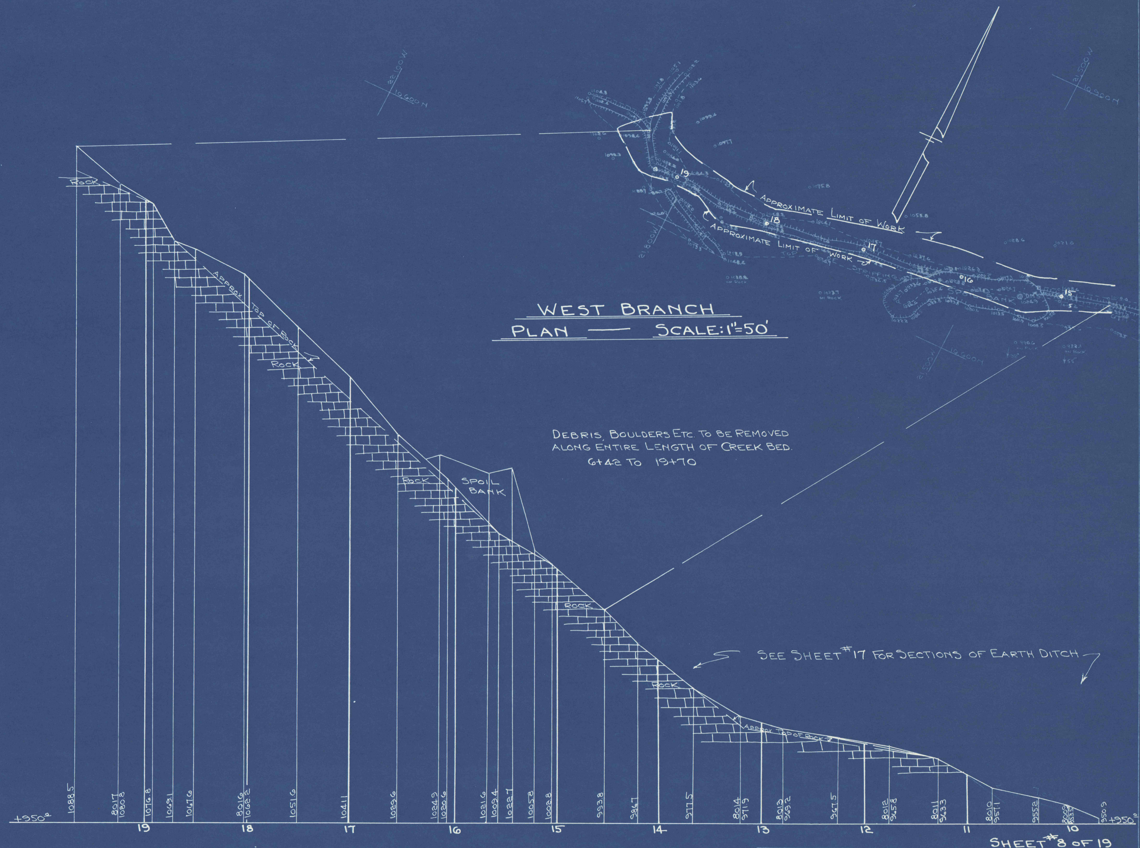
PROFILE ALONG C t OF DITCH SCALE: 1"=50' HOR. & 1"=10' VERT.
