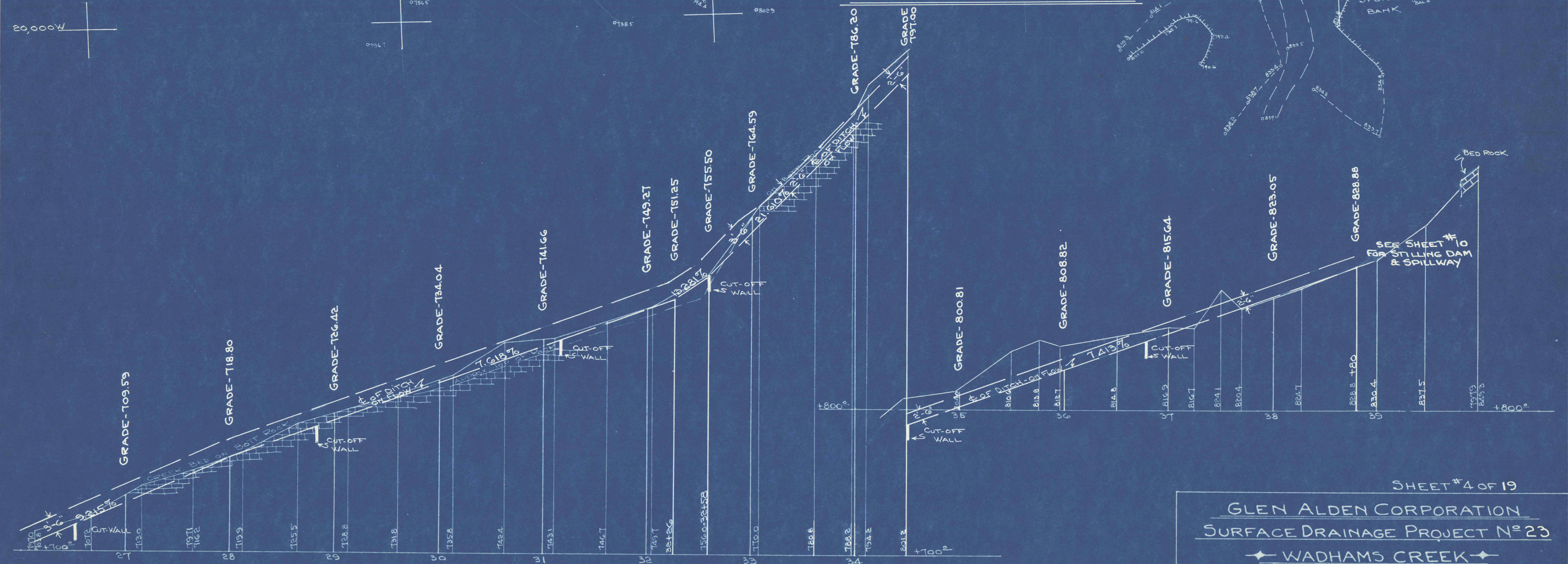
PROFILE ALONG C OF DITCH SCALE: 1"=50' HOR. & 1"=10' VERT.
