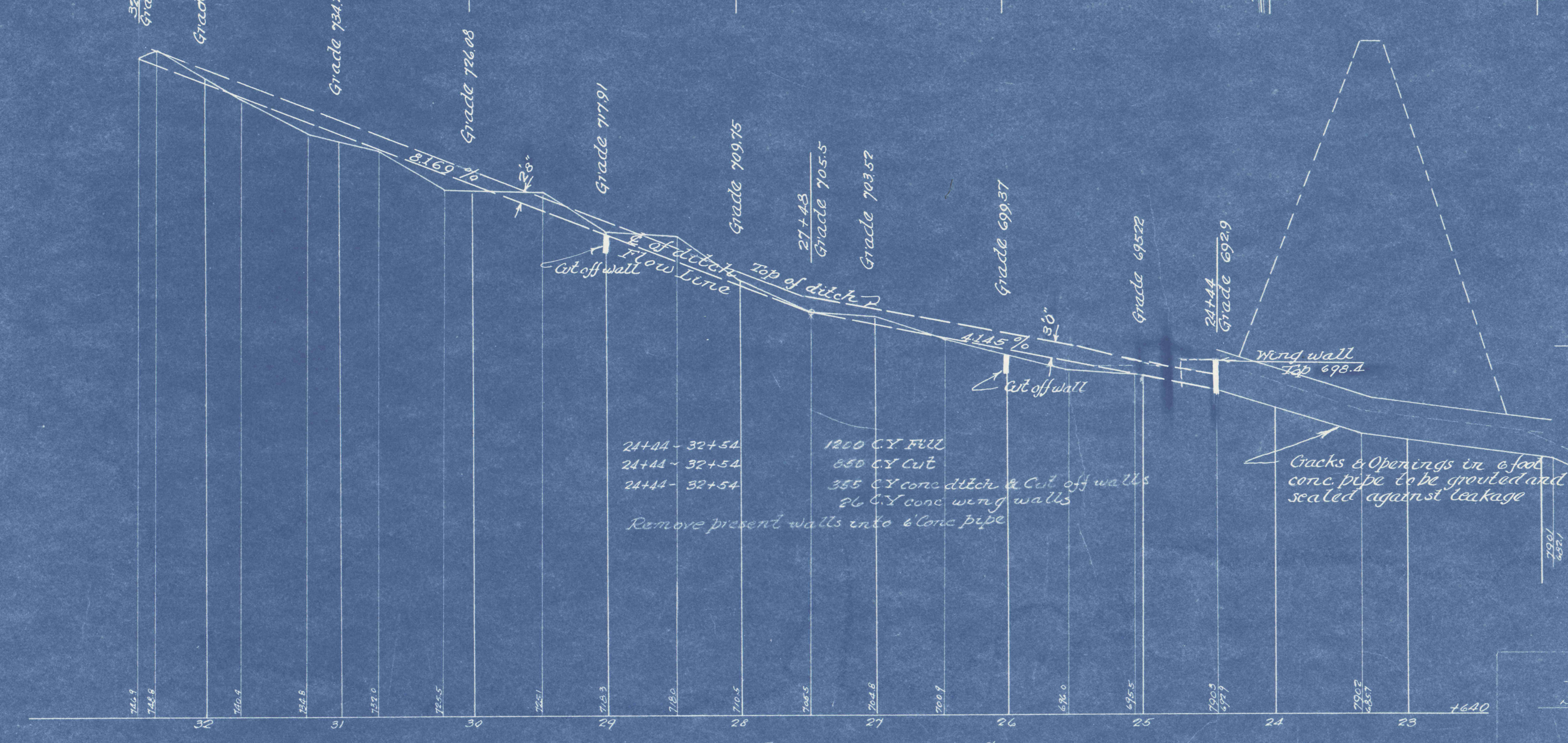
PROFILE ALONG C. OF DITCH Scale 1" = 50' Hor. & 1" = 10' Vert.
