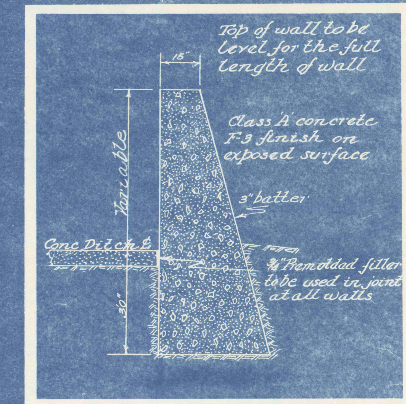
Typical Section of wing wall at E. of ditch
