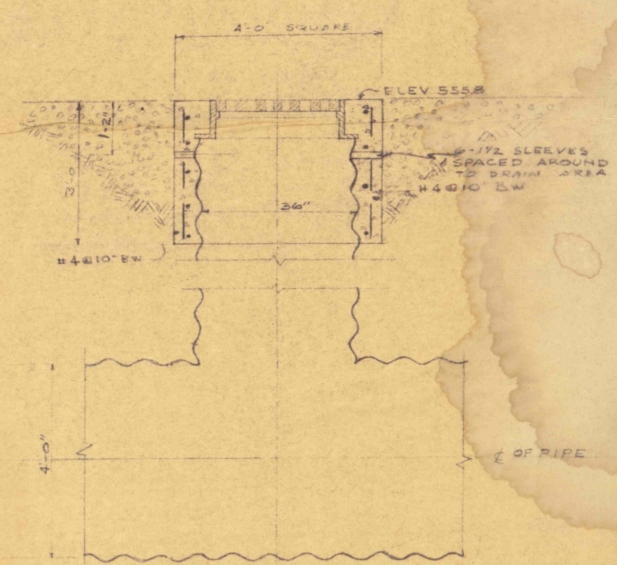
36" MANHOLE DETAIL NO SCALE
