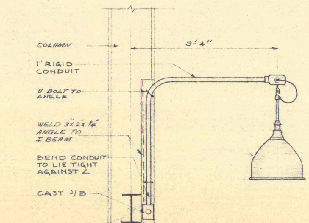
TYPE A LTG. FIX. MOUNTING NO SCALE
