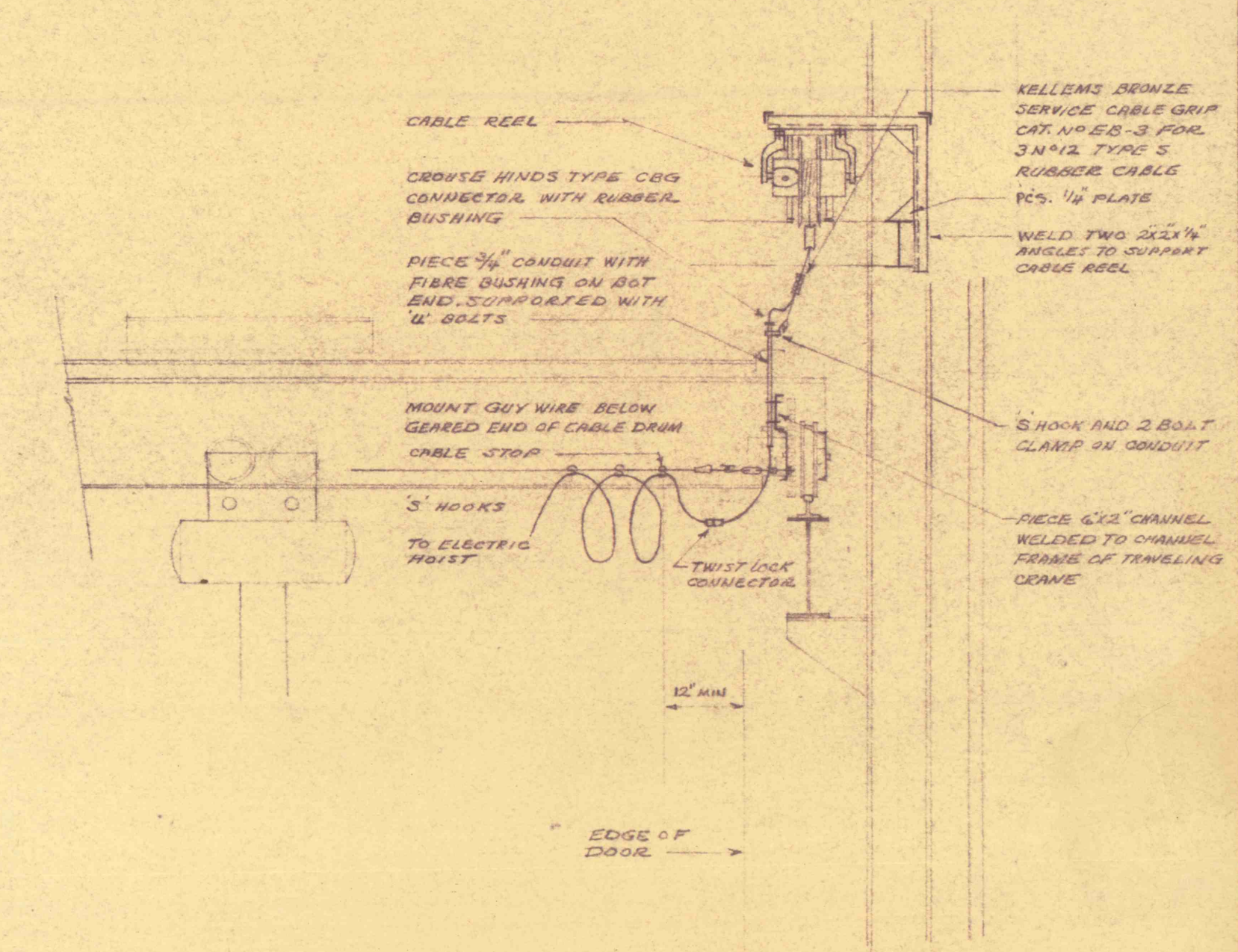
CRANE WIRING ARRANGEMENT APPROX. SCALE 3/8" = 1'-0"
