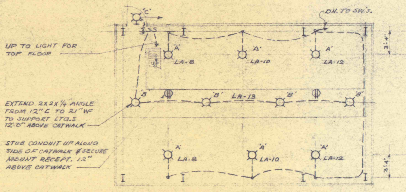
PUMP ROOM PLAN EL. 27'-6" SCALE 3/8" = 1'-0"
