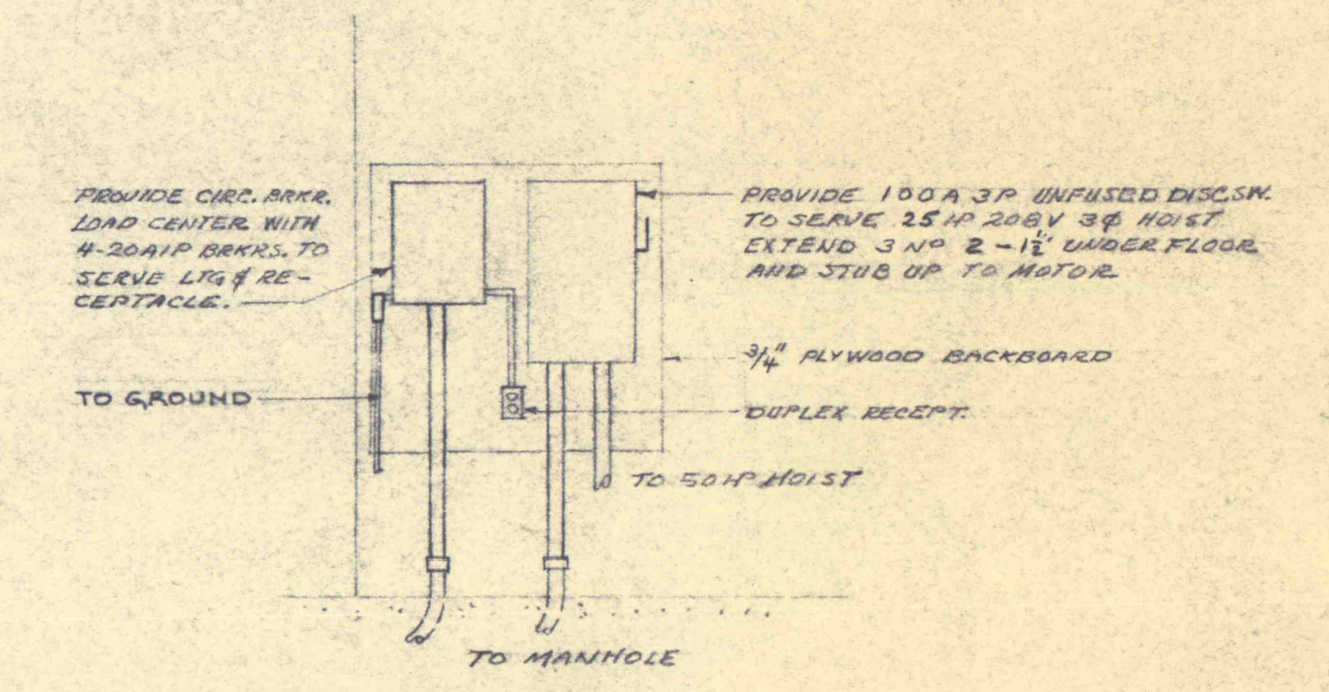
HOIST HOUSE BACKBOARD NO SCALE
