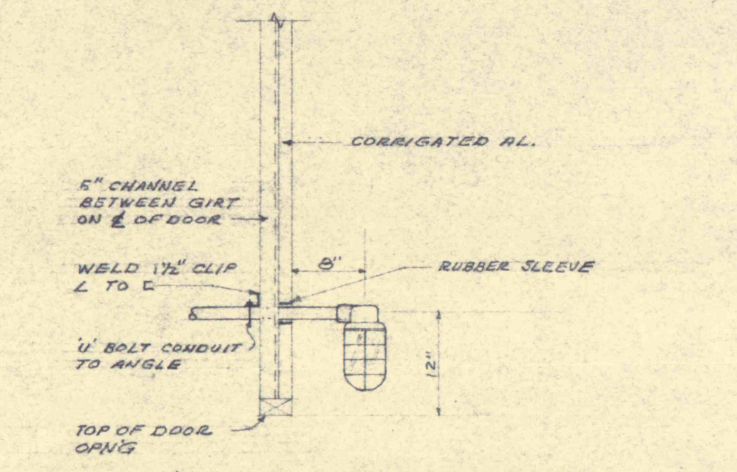
TYPE C' LTG. FIX. MOUNTING SCALE 3/4" = 1'-0"
