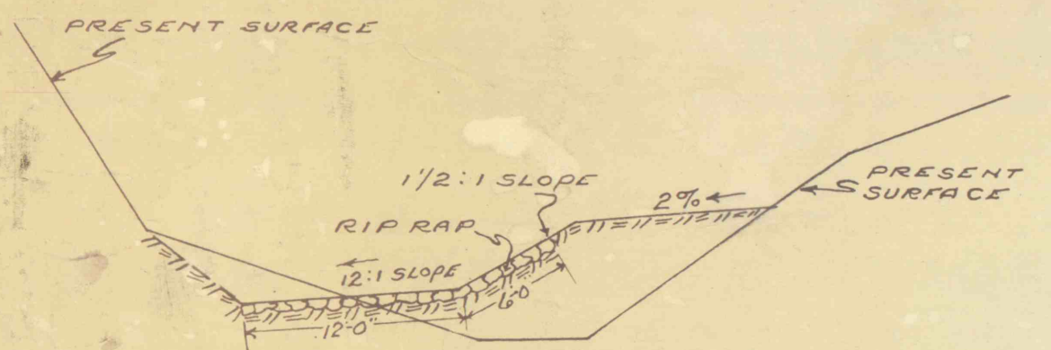
SECTION SHOWING RIP RAP ALONG CURVE ON SOUTH BRANCH N#2
