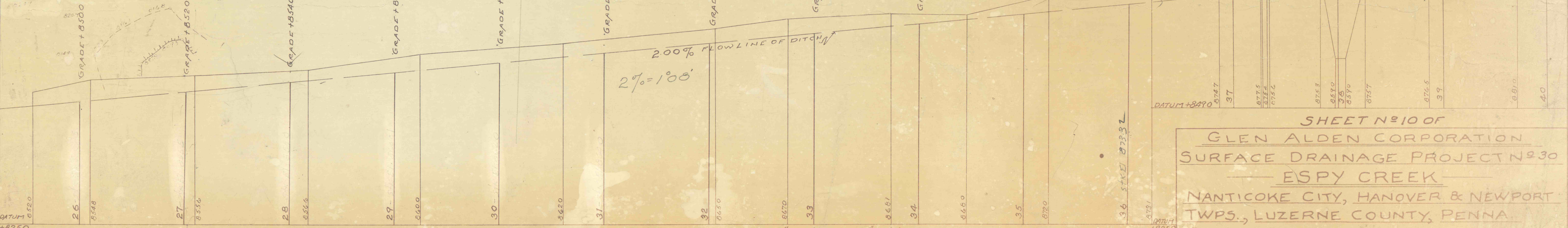
PROFILE ALONG E OF EARTH DITCH-LOOKING SOUTH-SCALE 1"=50' HOR-1"=10' VERT
