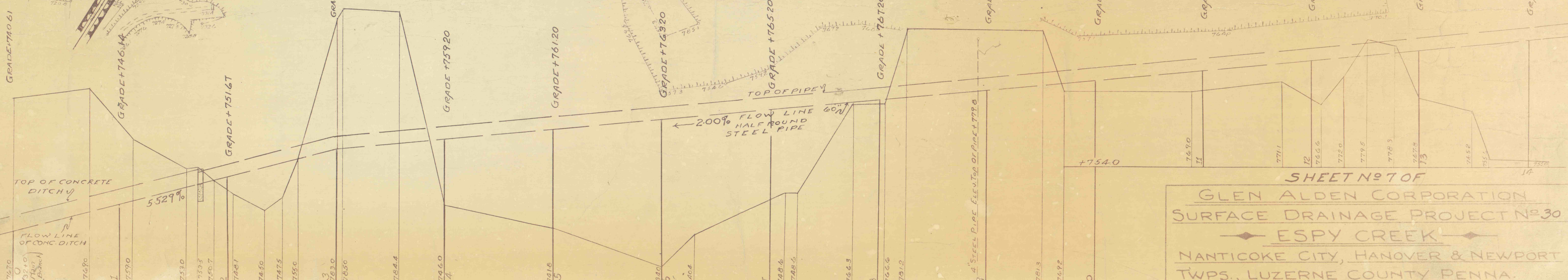
PROFILE ALONG C/L OF HALF ROUND STEEL PIPE - LOOKING SOUTH - HOR. SCALE 1"=50' - VERT. 1"=10'
