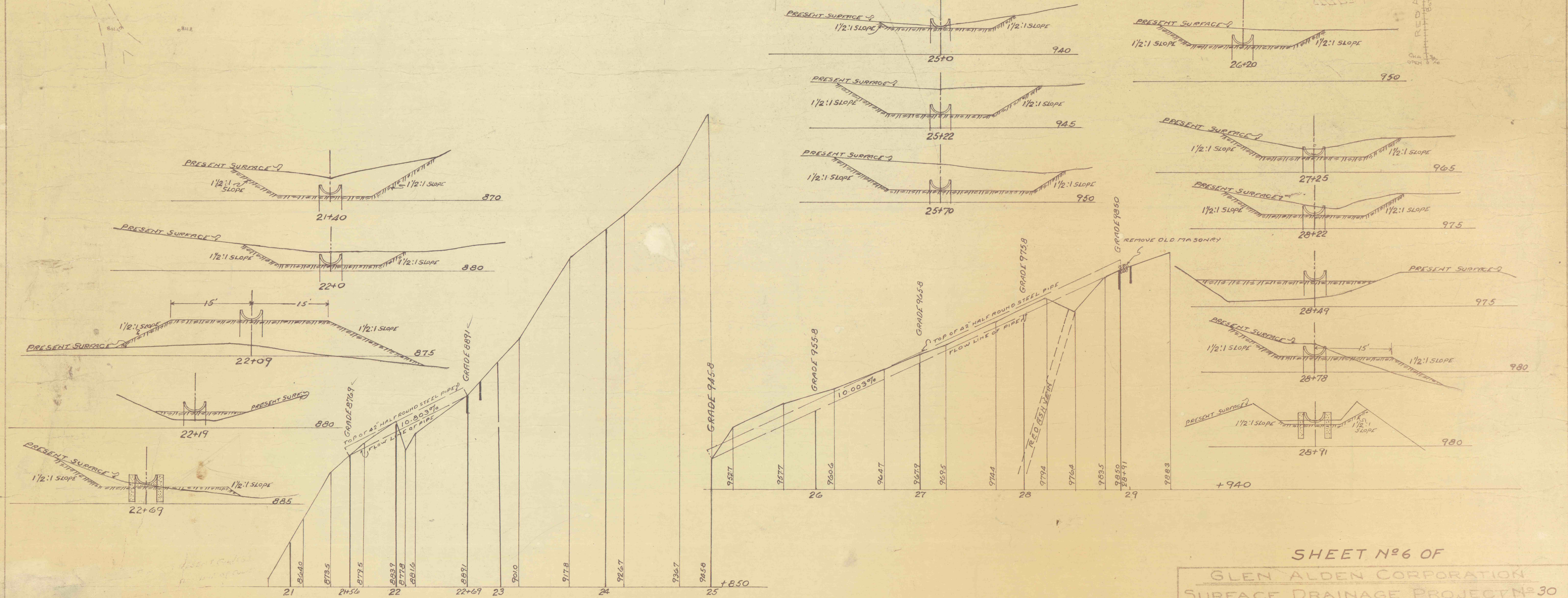
EAST BRANCH PROFILE ALONG C OF 42" HALF ROUND STEEL PIPE-LOOKING EAST. SCALE: HORIZ=50' VERT. 1"=10'
