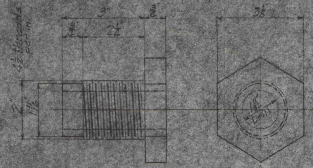
BRONZE STUFFING BOX BUSHING FINISH ALL OVER MARK ② 2-REQ. Scale: 6" = 12"
