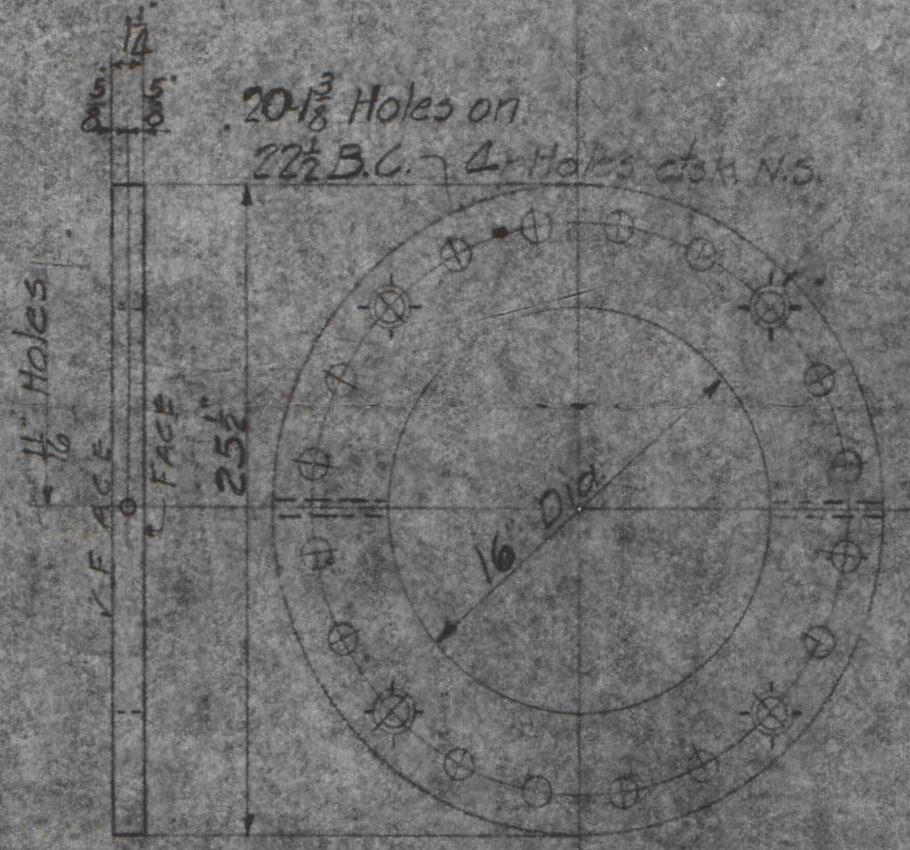
BRONZE RING FOR COOLING COIL SUPPORT MARK ③ 2-REQ. Scale: 1/2" = 12"
