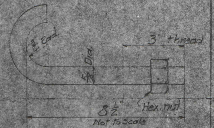
18-8 STAINLESS STEEL HOOK BOLT MARK ④ 4-REQ. Scale: 6" = 12"
