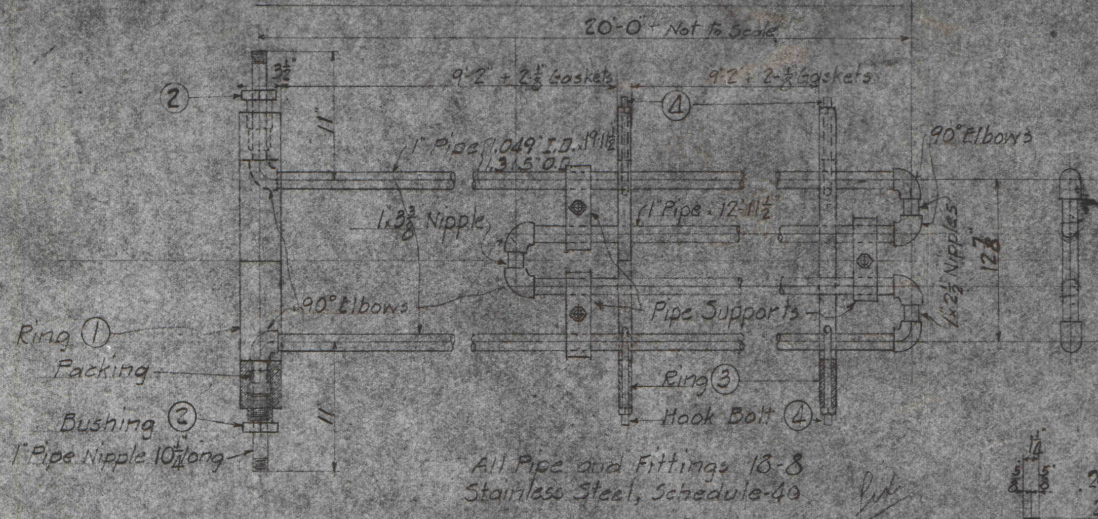
OIL COOLING COIL FOR 16" FLANGED PIPE Scale: 1/2" = 12"
