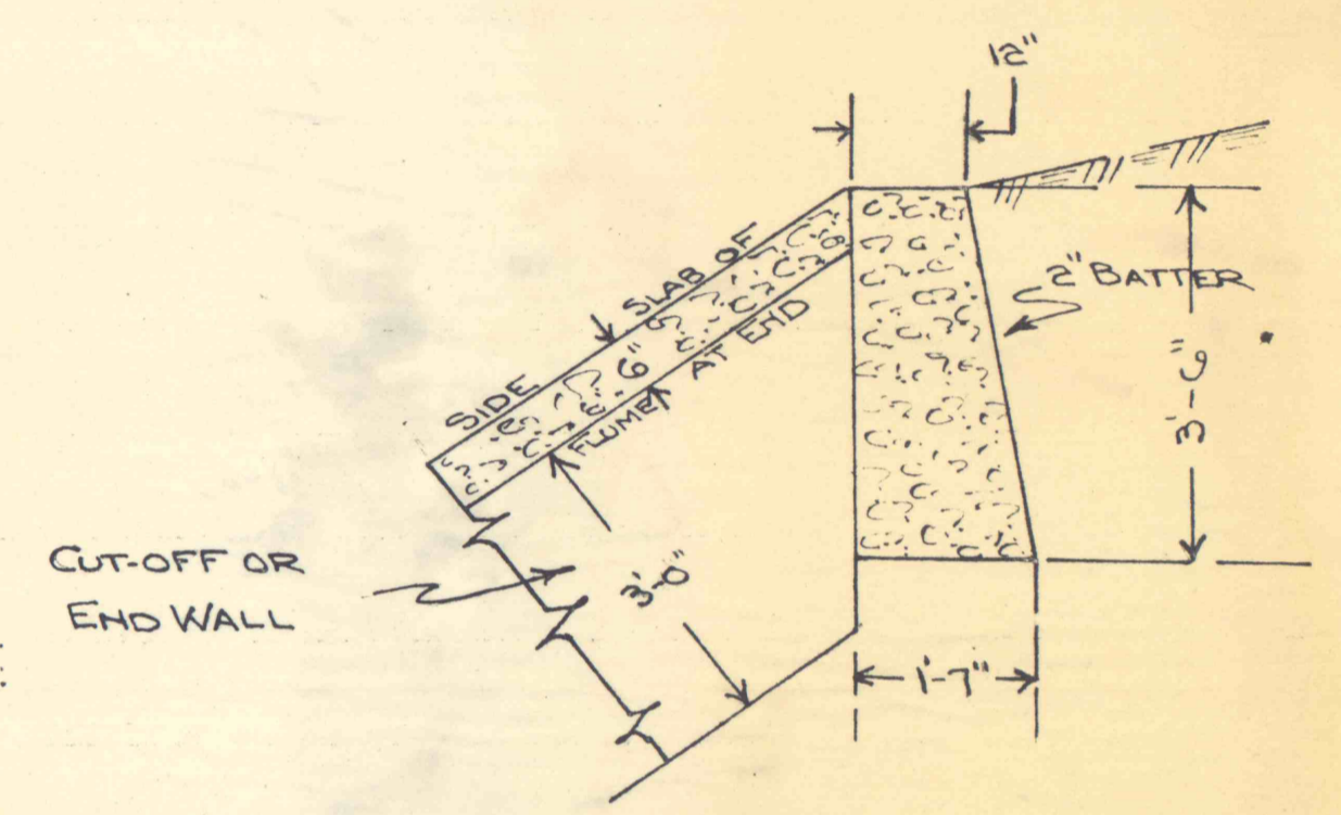
TYPICAL SECTION THROUGH WING WALLS SCALE: 1" = 2'
