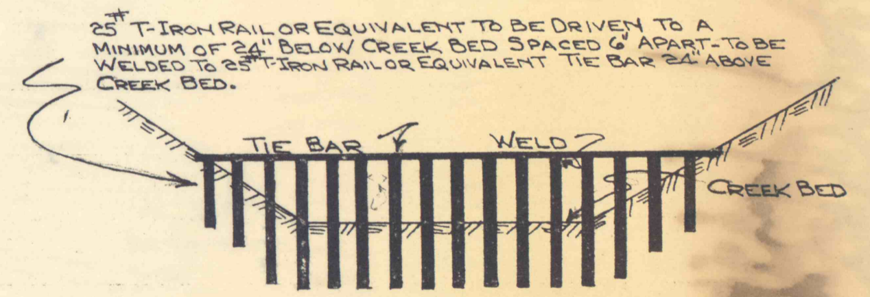
TYPICAL SECTION OF TRASH RACK TO BE INSTALLED 50' FROM THE END OF EACH SPUR & EAST & WEST BRANCHES - SCALE: 1" = 4'
