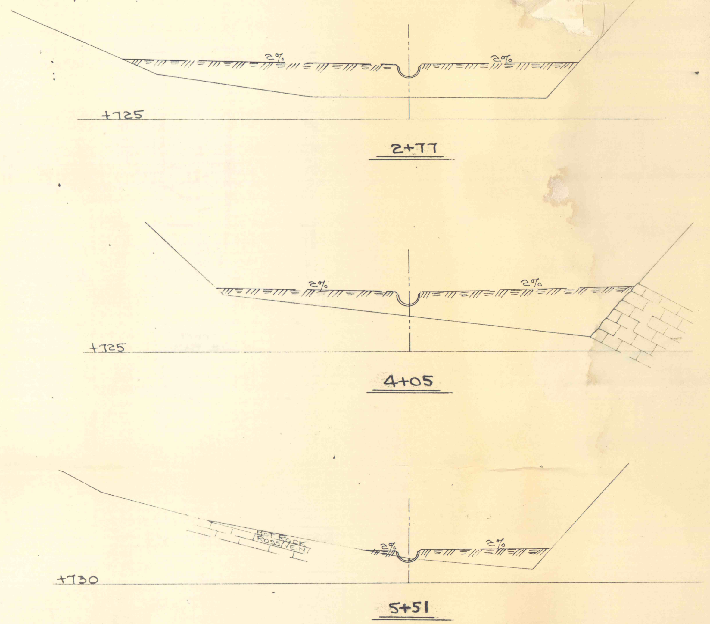
CROSS SECTIONS - SCALE: 1"=10'
