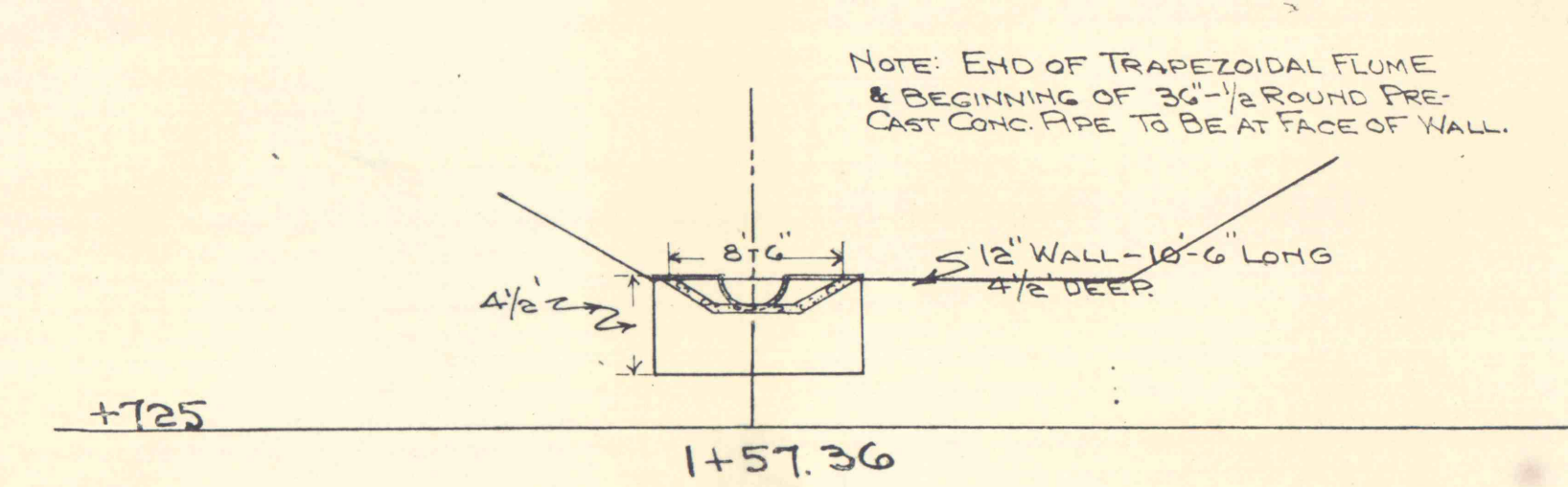
CROSS SECTIONS - SCALE: 1"=10'
