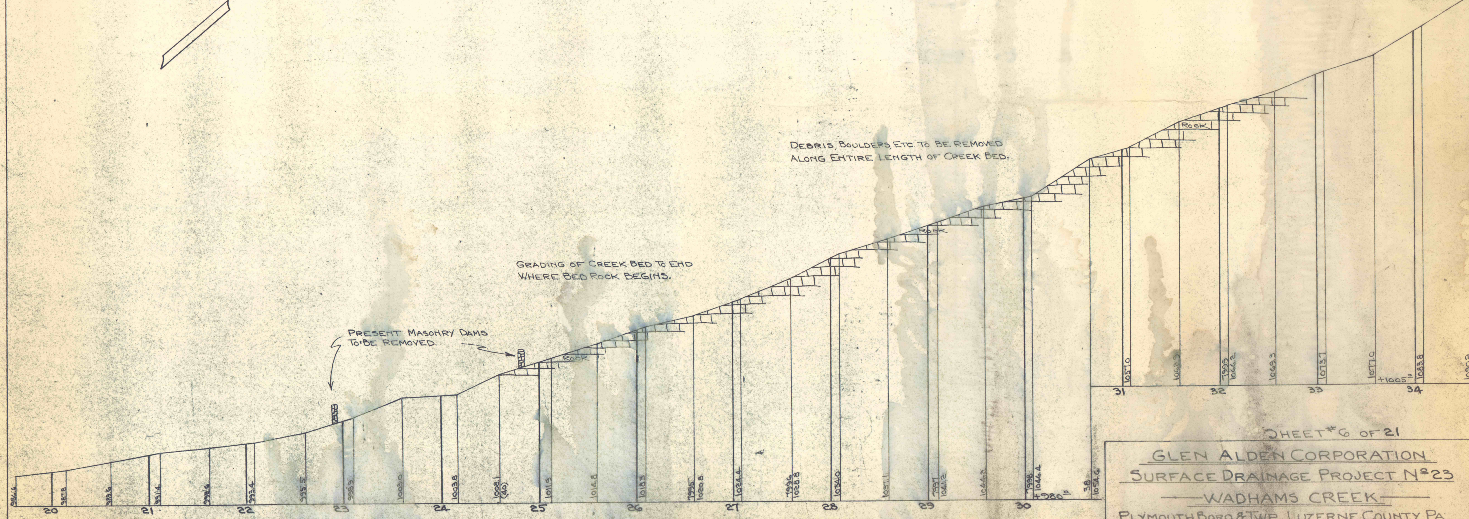
PROFILE ALONG \phi OF DITCH — SCALE: 1"=50' HOR. & 1"=10' VERT.
