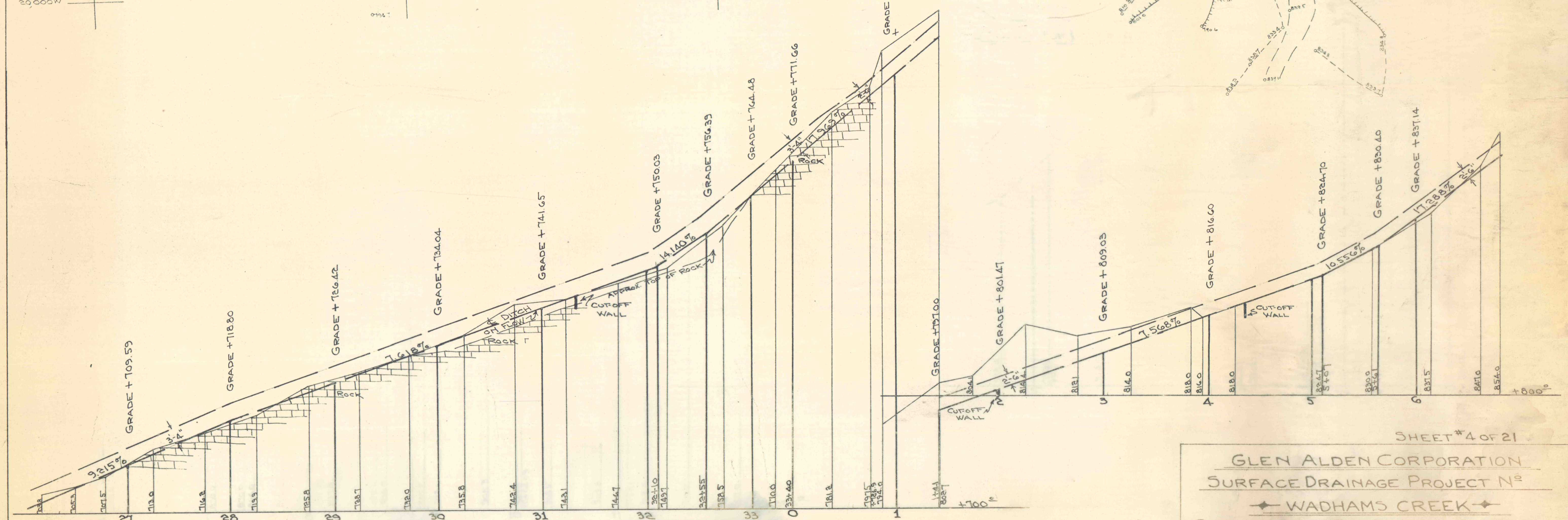
PROFILE ALONG \frac{1}{2} OF DITCH SCALE: 1" = 50' HOR & 1" = 10' VERT.
