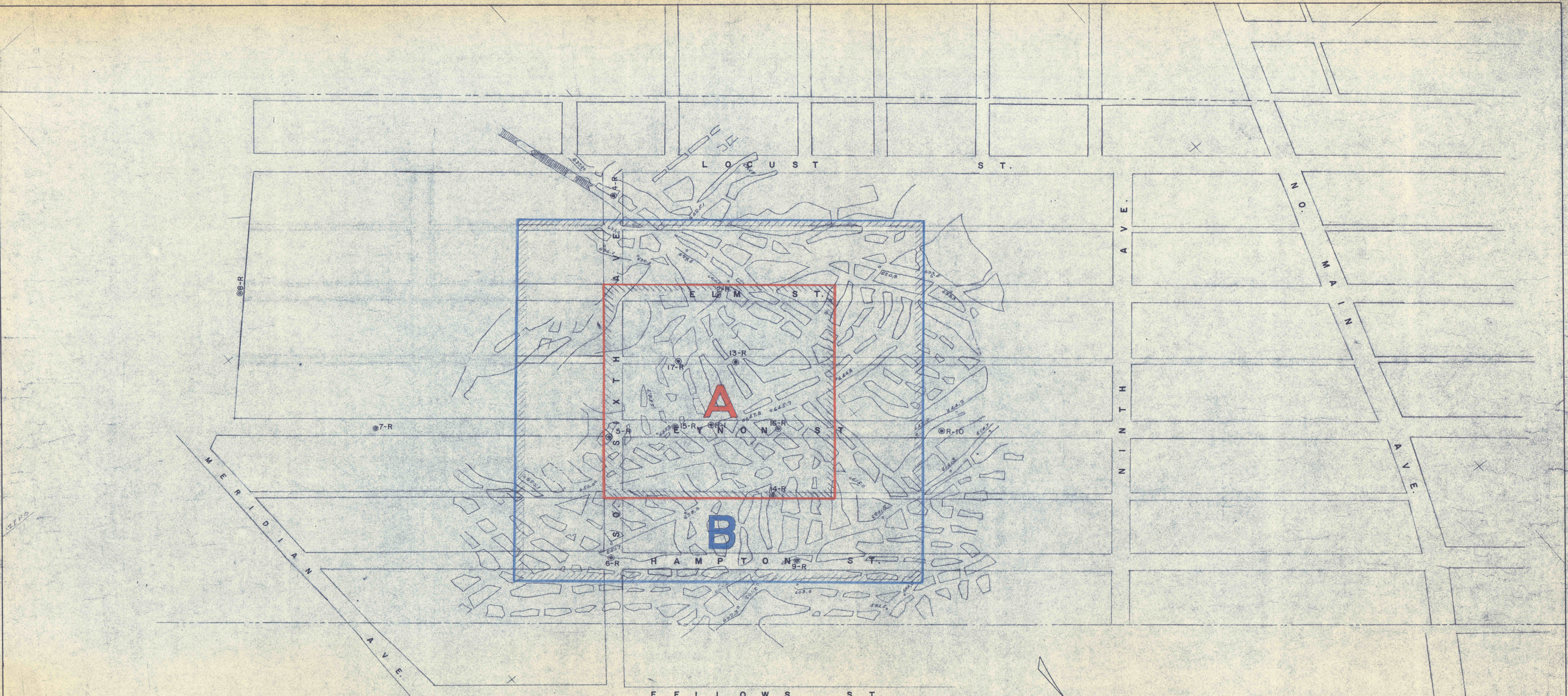
MAP SHOWING ROCK VEIN PROPOSED FLUSHING AREAS—TO CONTROL MINE FIRE BELLEVUE SECTION CITY OF SCRANTON, LACKAWANNA CO. PA. PUBLIC HEALTH & SAFETY PROJECT NO.9 PENNSYLVANIA DEPARTMENT OF MINES & MINERAL IND'S. SCALE—1"=100' JULY 1964
