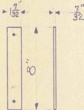
Hubbard Stock No. 7570 Galvanized Pole Shim.
