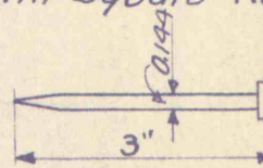
Hubbard Stock #8260, 10d. "Copperweld" Nail. FOR STRAIN PLATES, & POLE SHIMS
