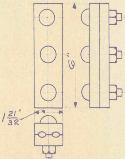
Hubbard Stock No. 7461 Galvanized Heavy Type 3 Bolt Guy Clamp.
