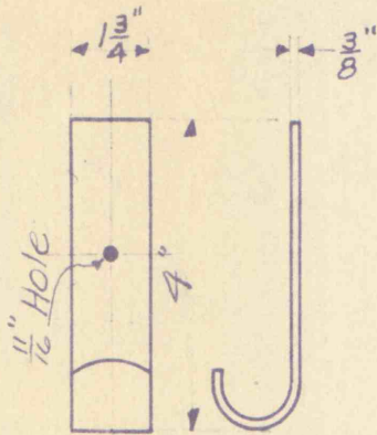
Hubbard Stock No 7584 Galvanized Guy Hook
