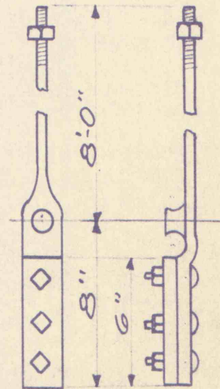
Hubbard Stock No. 6428 - Gould's Clamp Anchor Rod - \frac{3}{4} " Dia. 8'-0" Long. with Square Nut and 3-Bolt Clamp
