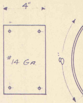
Hubbard Stock No 7575 Galvanized Steel Strain Plate.
