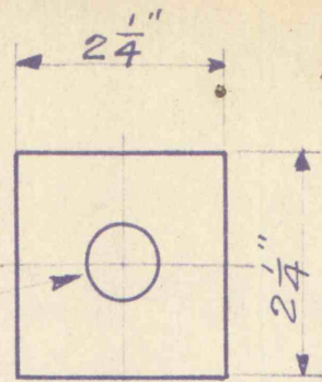
Hubbard Stock No. 7814 2\frac{1}{4} " x 2\frac{1}{4} " Galvanized Square Washer, \frac{3}{16} " Thick, with \frac{13}{16} " Hole
