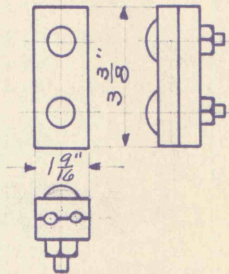
Hubbard Stock No. 7448 Galvanized Rolled Steel 2-Bolt Guy Clamp.
