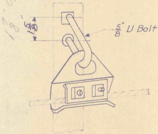
Hubbard Stock No. 6460 Flexible Ground Wire Clamp Hot Galvanized.
