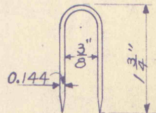
Hubbard Stock #7495 "Copperweld" Staple For fastening Ground Wire to Pole
