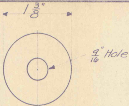
Hubbard Stock No. 7803 1\frac{3}{8} " Dia. \frac{7}{64} " Thick, Galvanized Round Washer with \frac{9}{16} " Hole.
