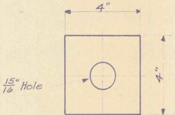
Hubbard Stock No. 7819 4" x 4" Galvanized Square Washer \frac{1}{4} " Thick with \frac{15}{16} " Hole
