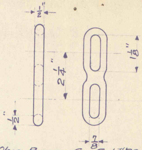
Ohio Brass Co. Cat. #72451 Galvanized Straight Strain Link
