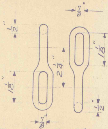
Ohio Brass Co. Cat. #72452 Galvanized Twisted Strain Link
