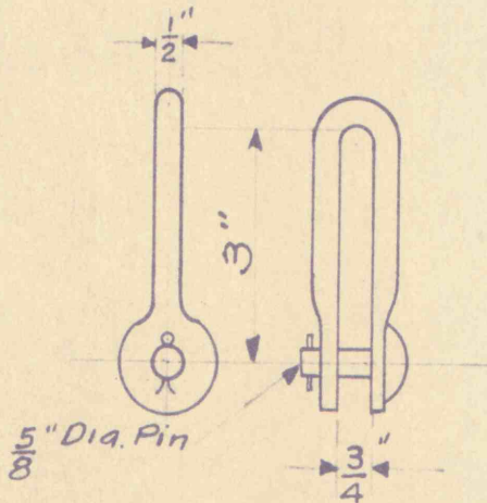
Hubbard Stock #6800 Galvanized Drop Forged Clevis
