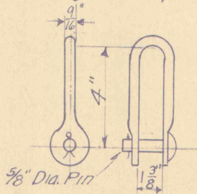
Hubbard Stock #6799 Galvanized Drop Forged Clevis.
