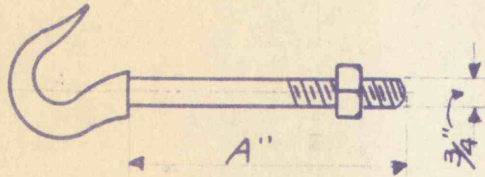
HUBBARD DROP FORGED HOOK BOLT
