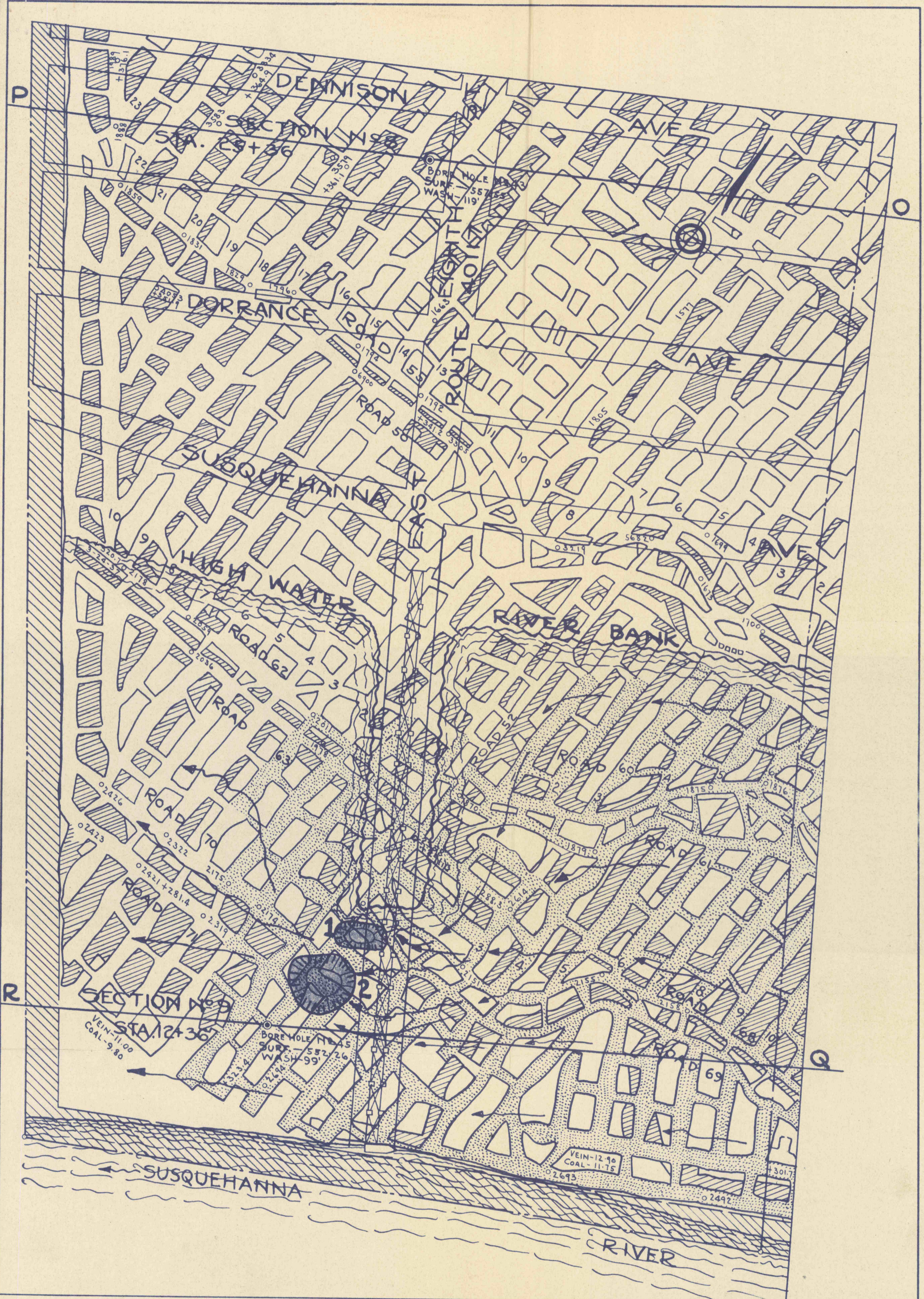
MAP SHOWING PORTION OF PITSTON VEIN OF THE DIAL ROCK COAL COMPANY UNDER ROUTE 40117 WYOMING BORO.—LUZERNE COUNTY SCALE 1"=100'
