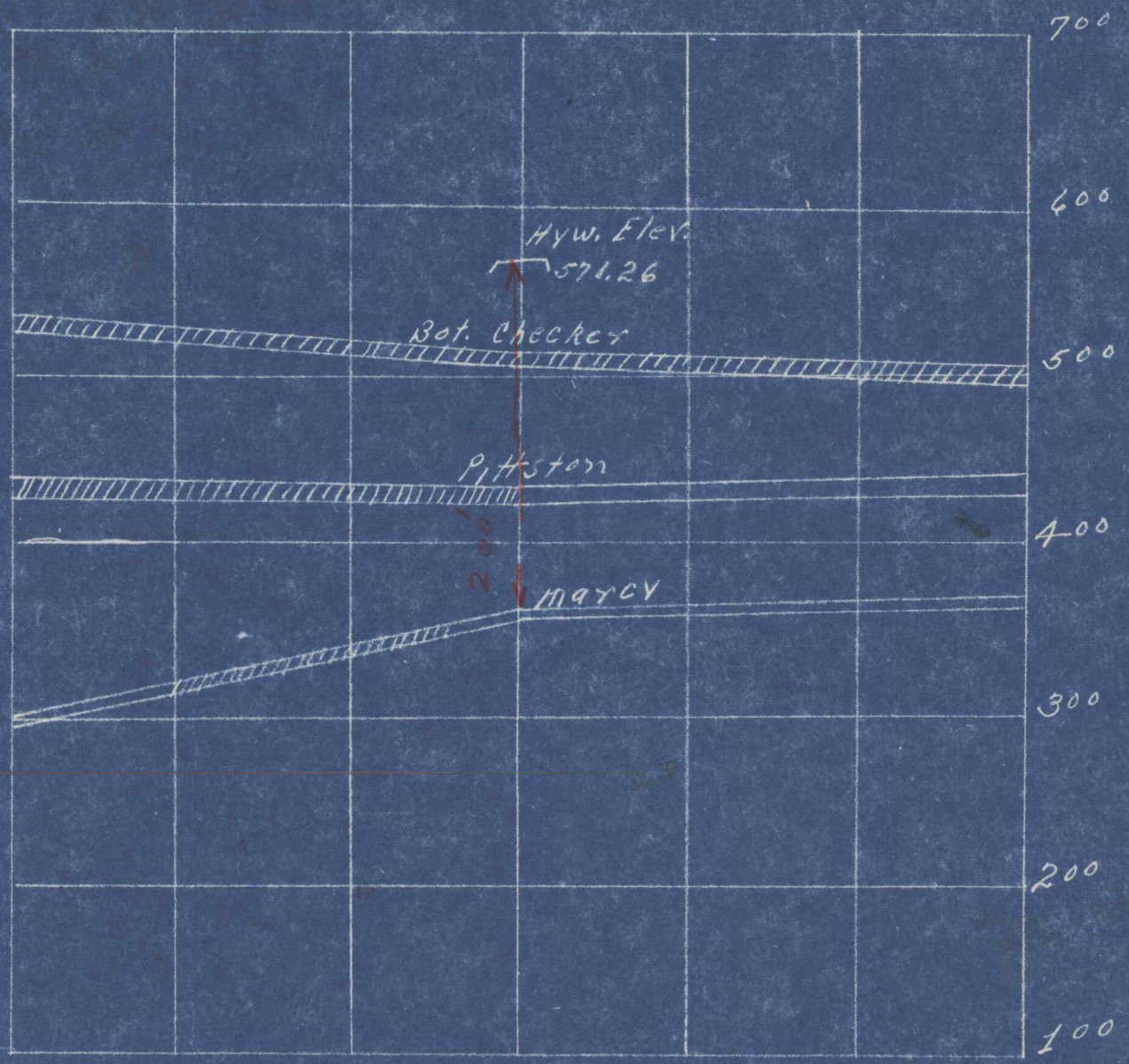
NO. 14 COLLIERY No. 14 Drifts- Marcy Vein Scale 1"-100' Cross section of Marcy Vein underlying Leg. Route #40038 in Plains Twp., Luz. Co. Pa. [Hatched Box] Virgin coal [Horizontal Hatched Box] First mining [Diagonal Hatched Box] Complete mining.
