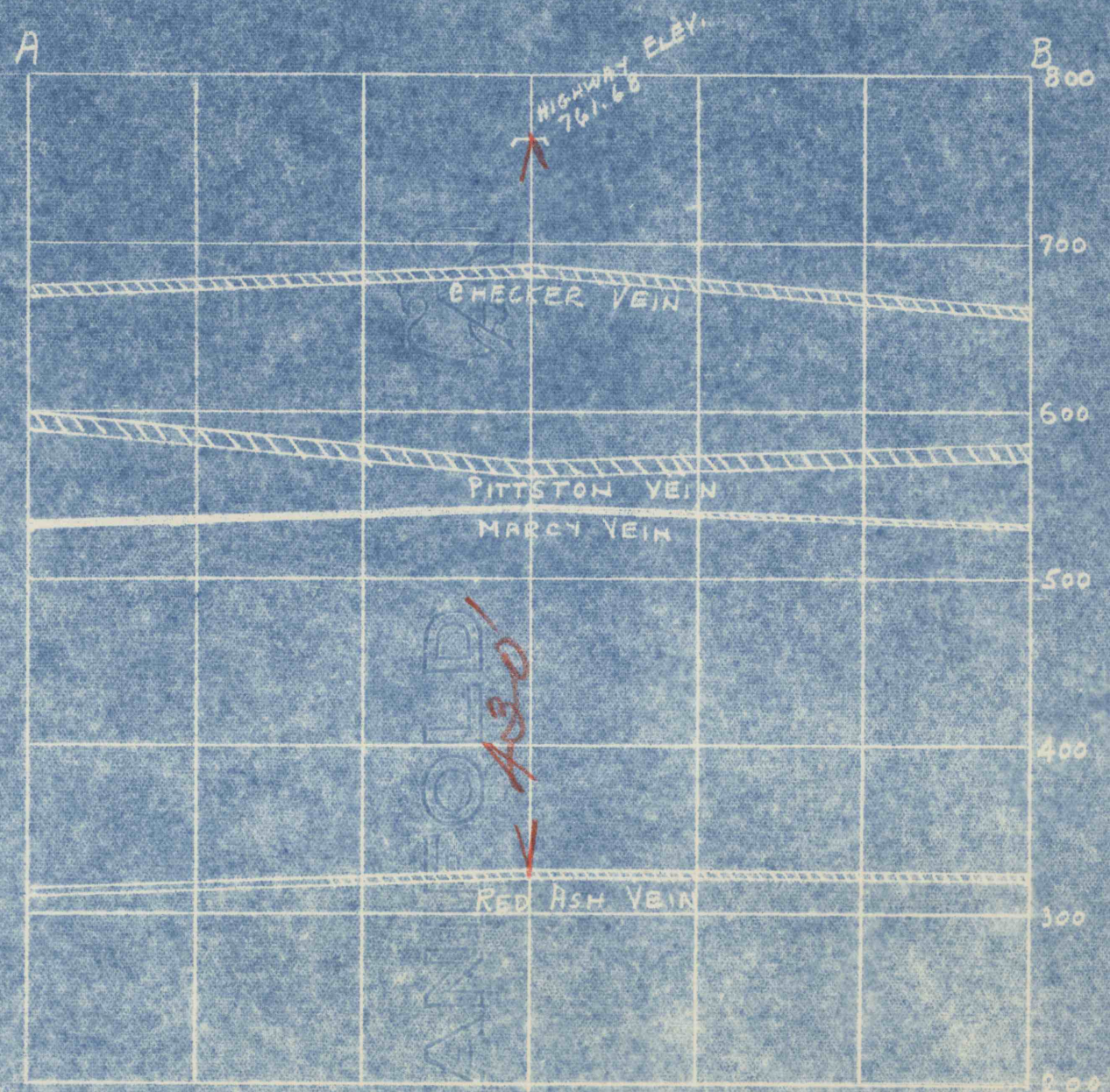
EWEN COLLIERY NO. 4 SHAFT - RED ASH VEIN Scale 1" = 100'
