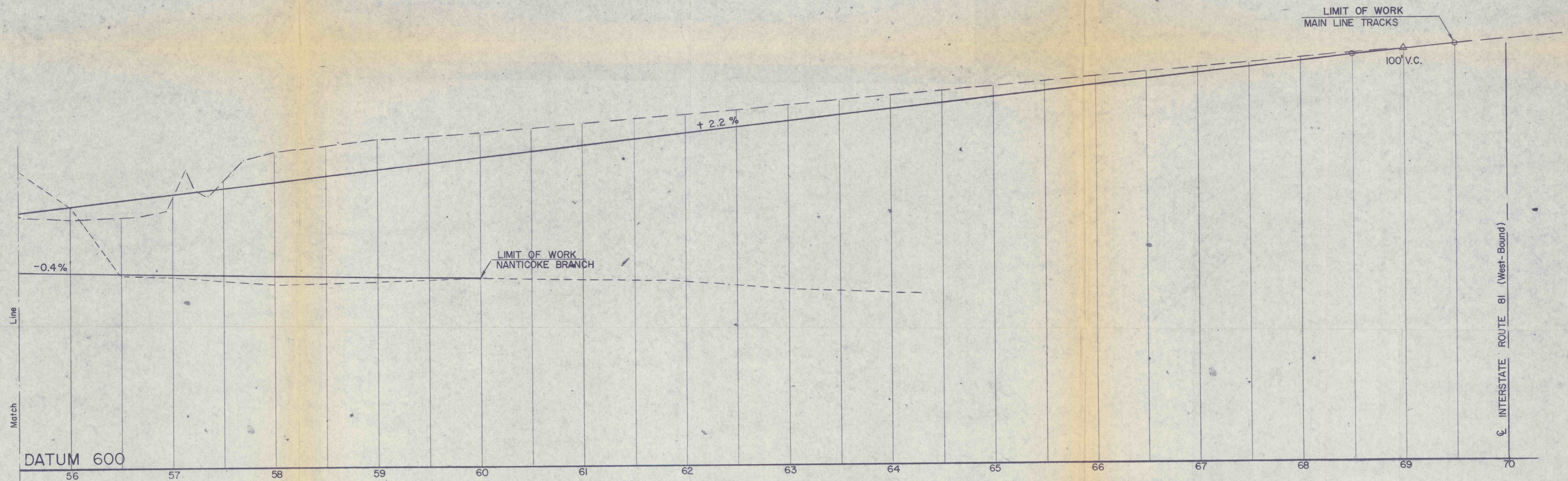
☉ PROFILE REVISION for MAIN LINE TRACKS & NANTICOKE BRANCH of CENTRAL RAILROAD of NEW JERSEY (ALTERNATE - 1)
