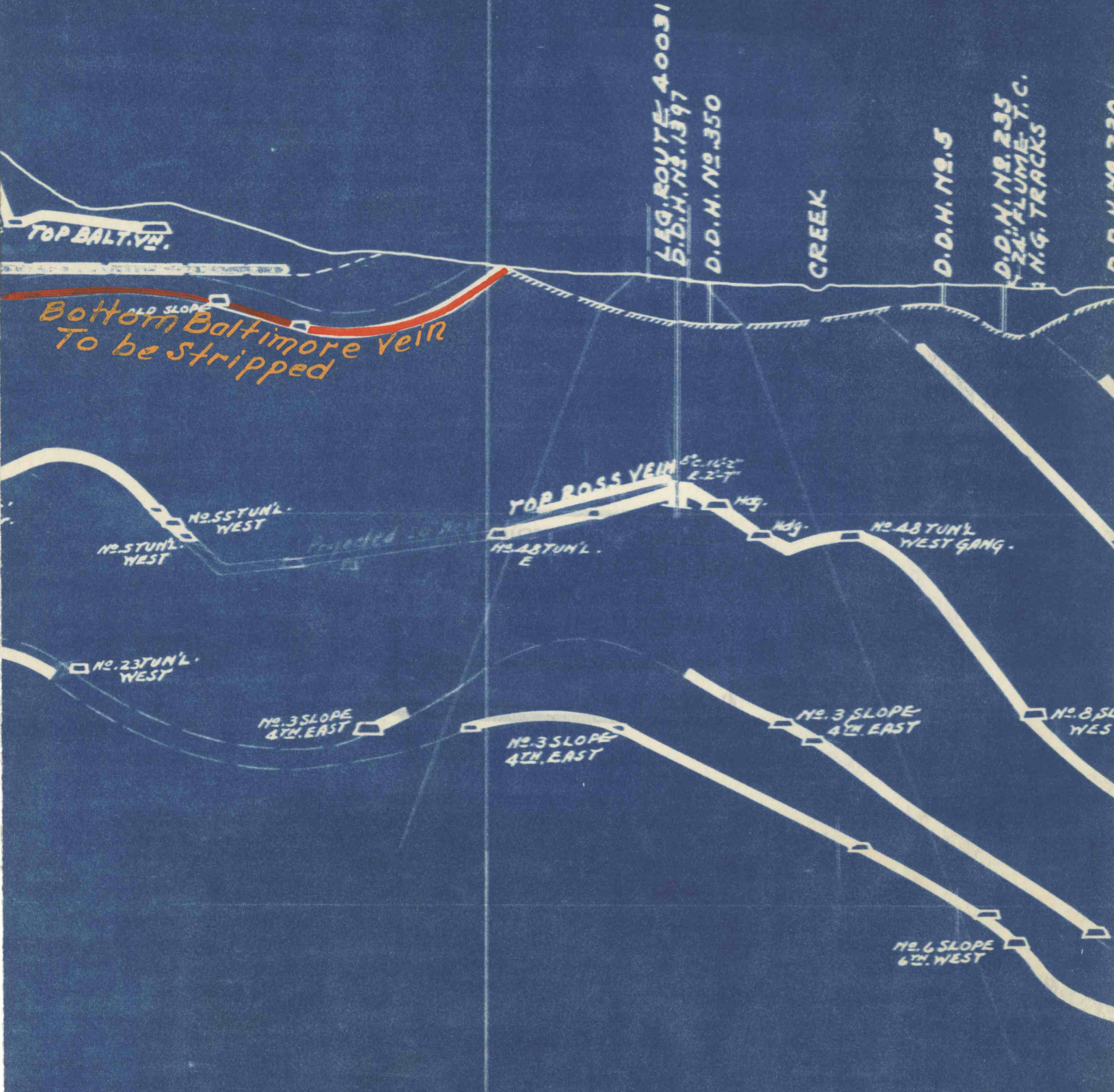
Wanamie No. 18 Colliery Cross Section F-146-2 Scale 1" = 100'
