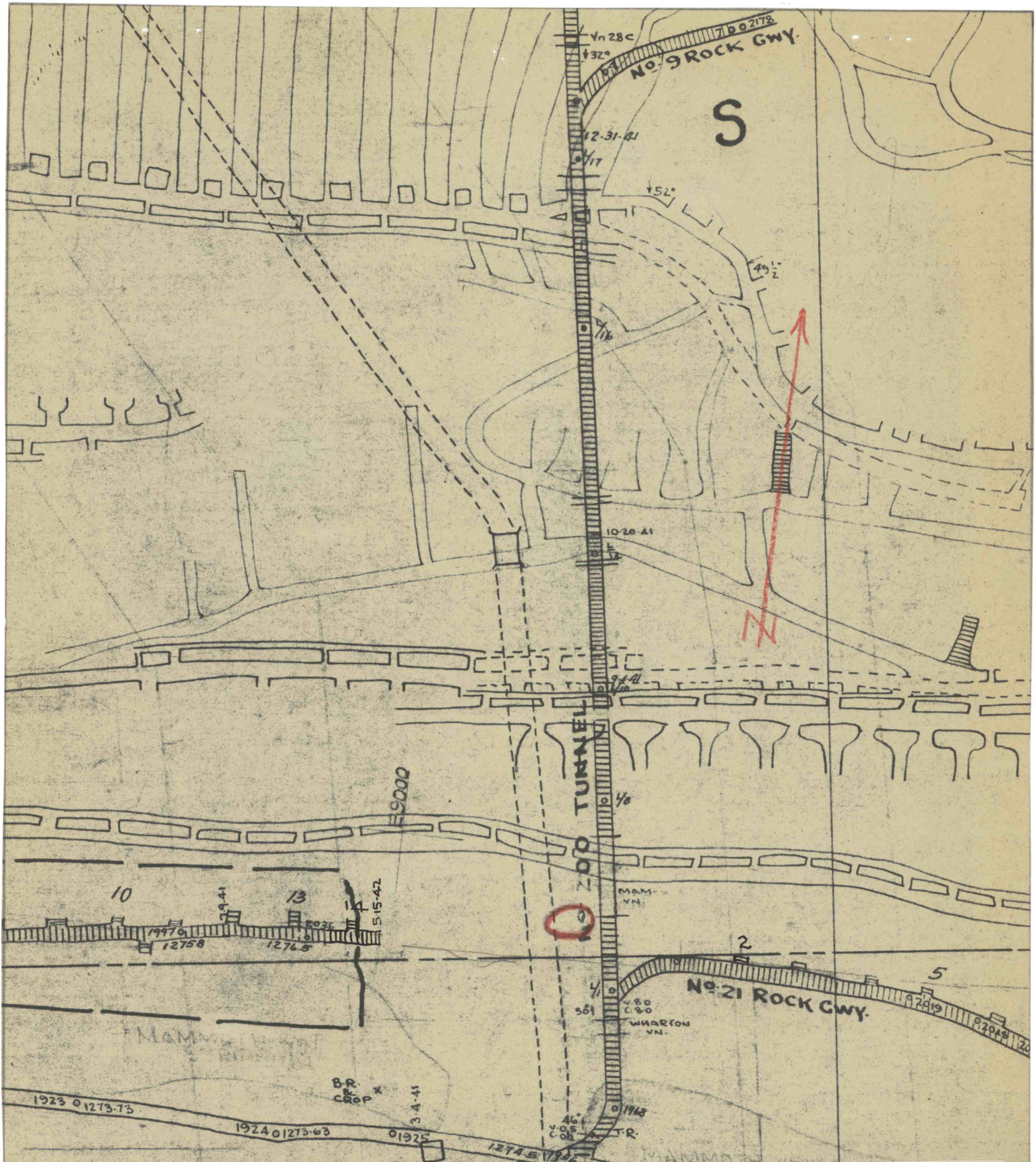
print of the Mammoth Vein showing cave in the Stockton Highway. Engr. Dept., L.V.C.Co., Hazleton, Pa. Scale 1" = 100' 5-15-42
