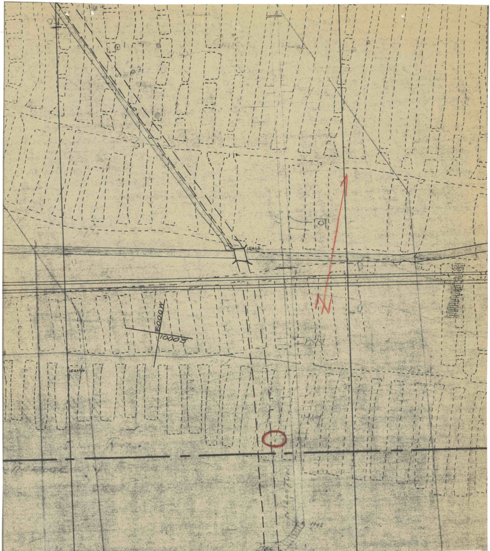
Print of the Primrose Vein showing cave in Stockton Highway. Engr. Dept., L.V.C.CO., Hazleton, Pa. Scale 1" = 100' 5-15-42
