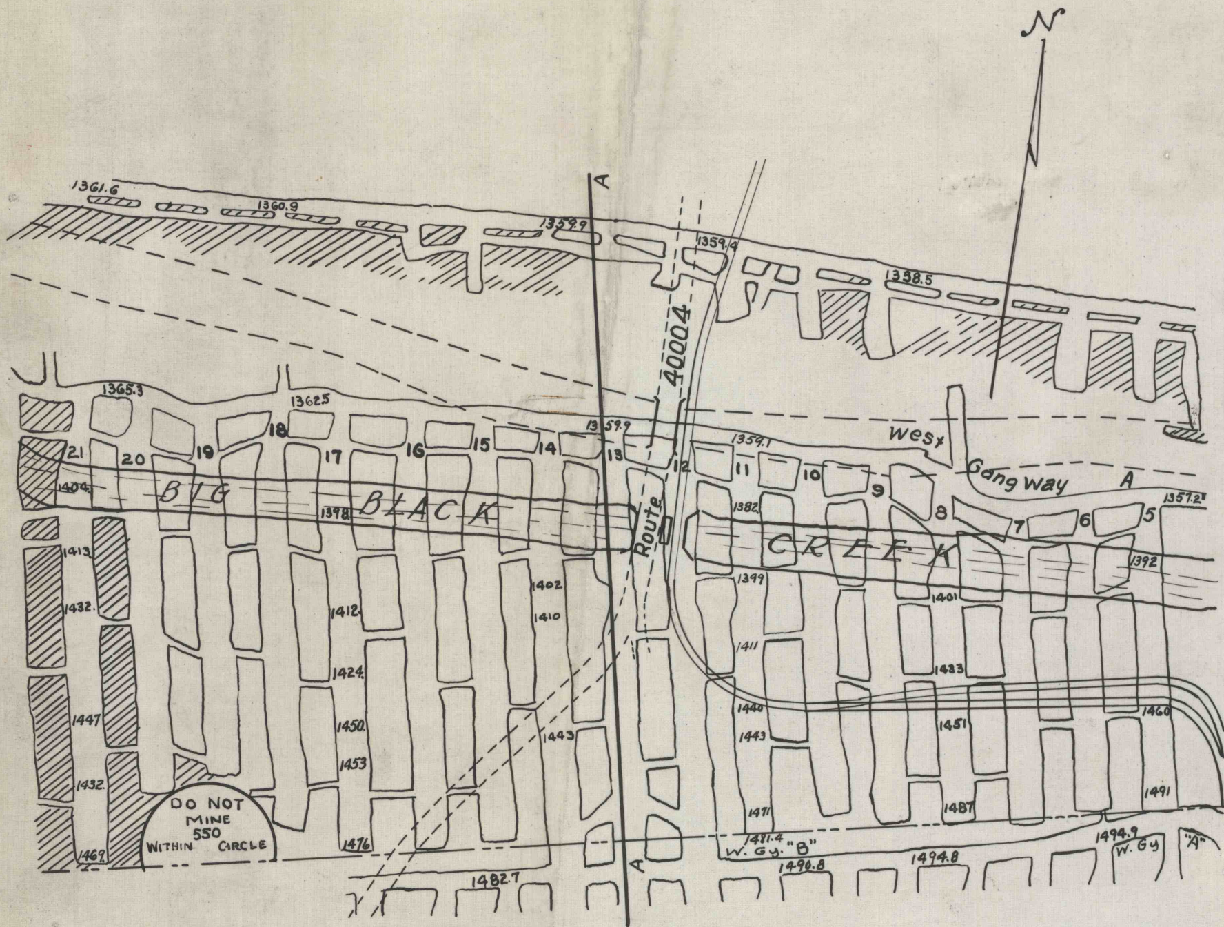
BUCK MOUNTAIN BED JEDDO HIGHLAND COAL CO. SCALE 1" = 100' APR. 8, 1937.
