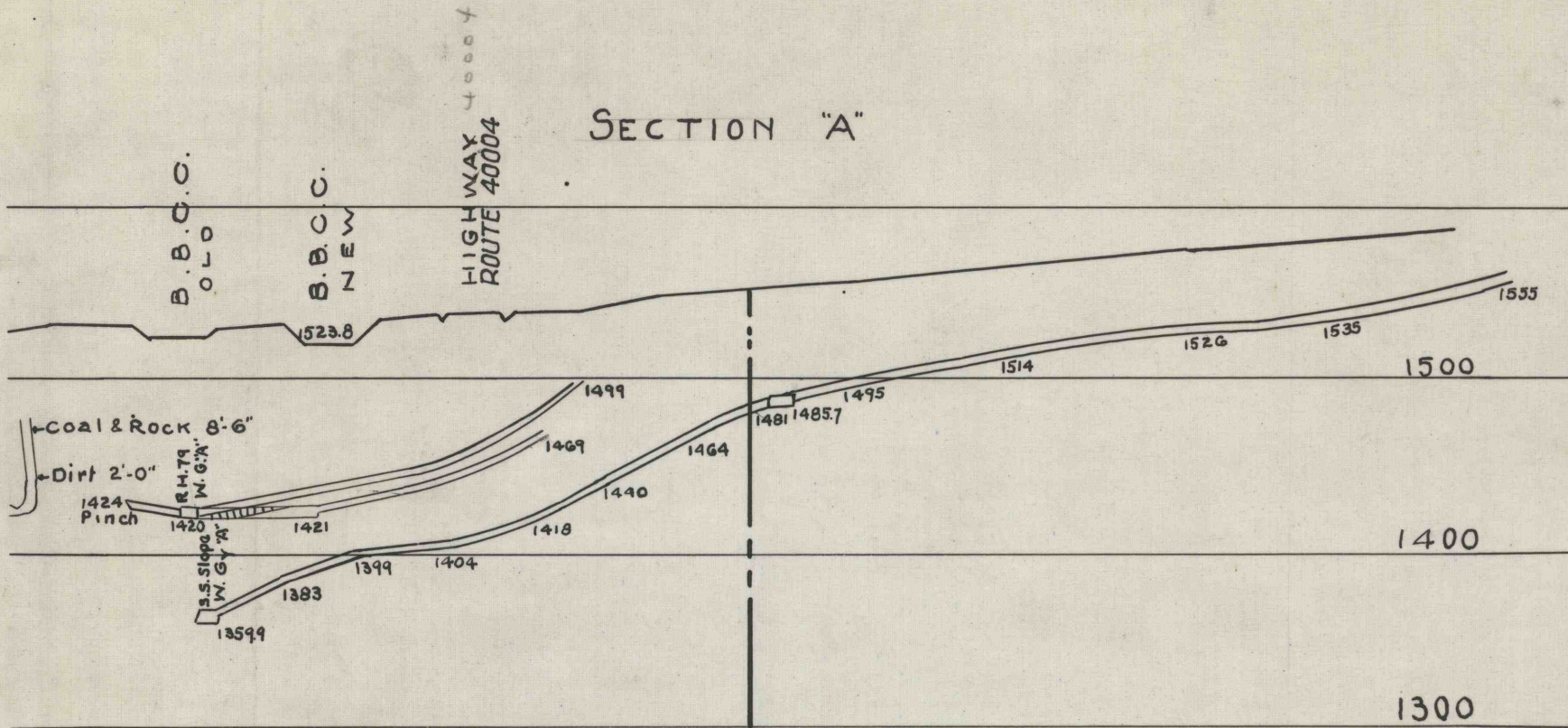
CROSS SECTION SHOWING POSITION OF COAL BEDS UNDER ROUTE 40004 AT OAKDALE LUZERNE CO. SCALE 1"=100 FT. APRIL 8, 1937.
