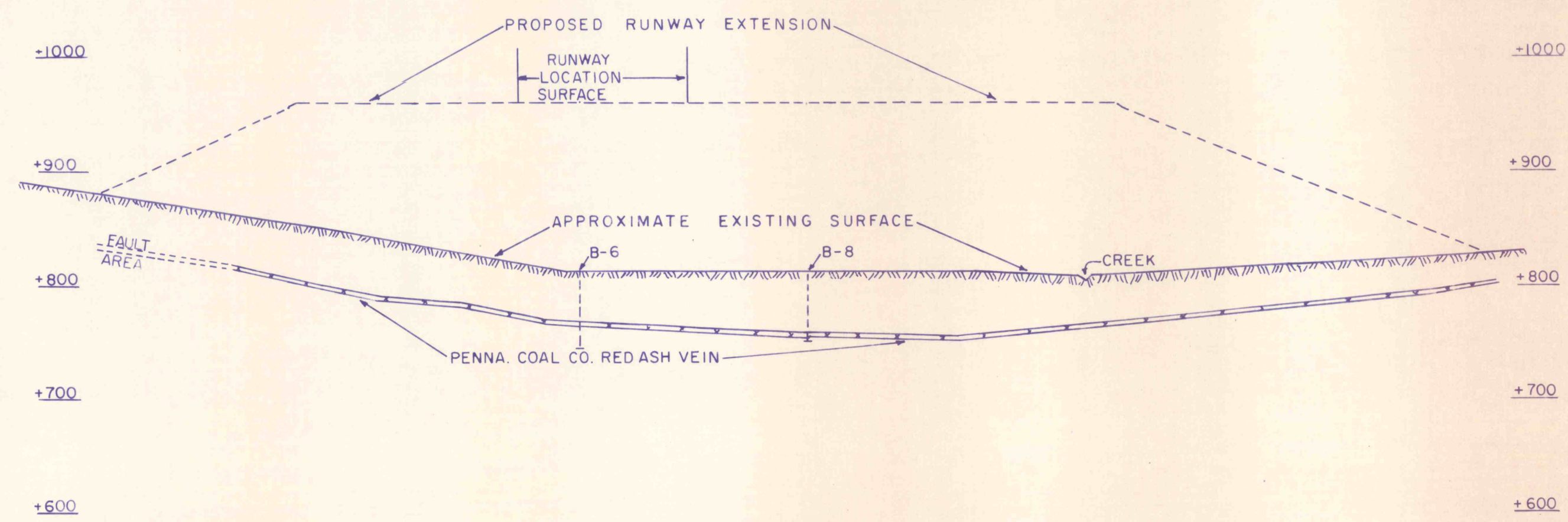
CROSS SECTION "B"- "B" APPROXIMATE VERTICAL CROSS SECTION LOOKING NORTHEAST SHOWING MINED COAL VEIN WITH RELATION TO THE SURFACE
