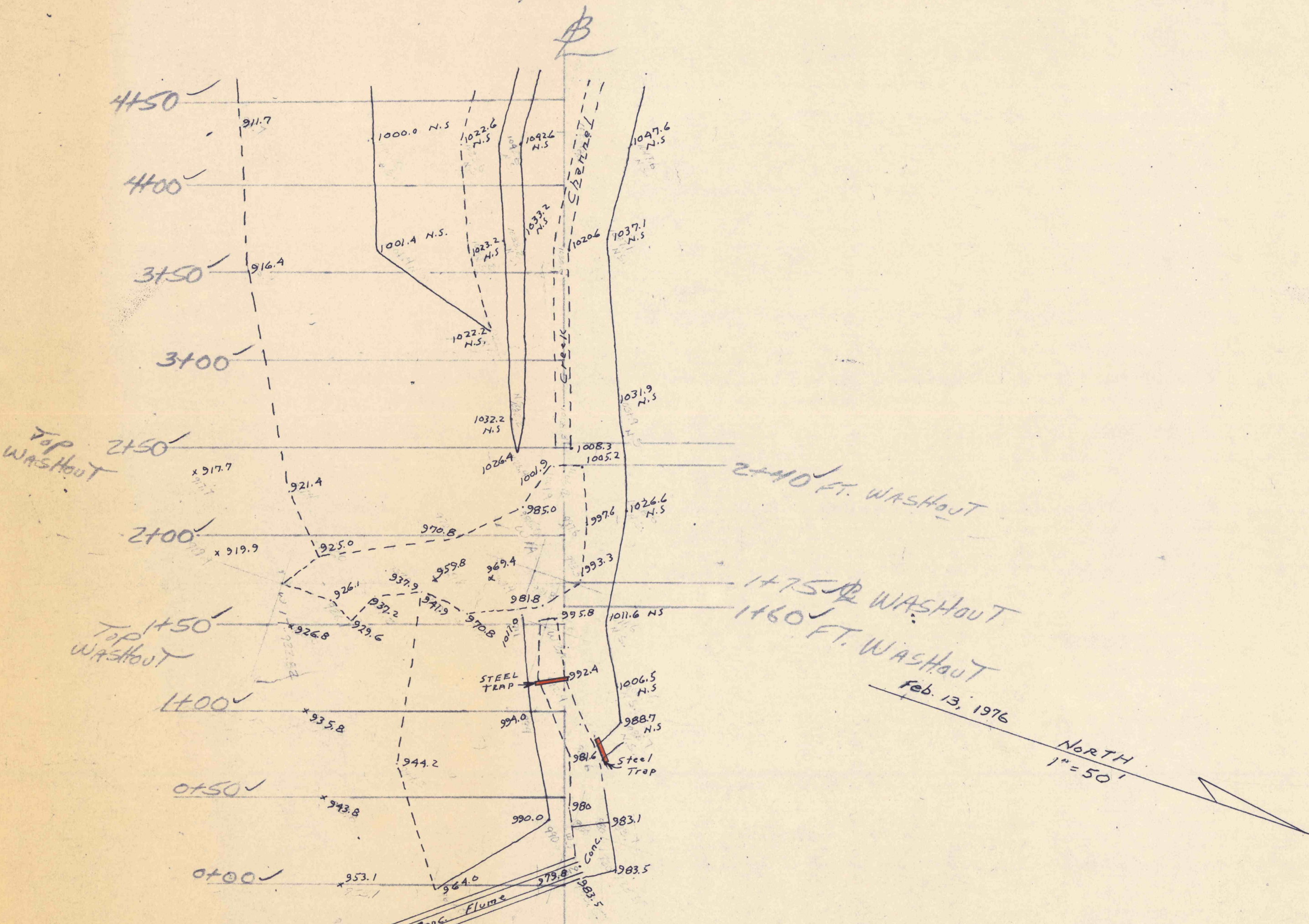
WADHAMS CREEK FLUME PLYMOUTH TWP. PENNSYLVANIA SCALE 1" = 50' FEB. 13, 1976
