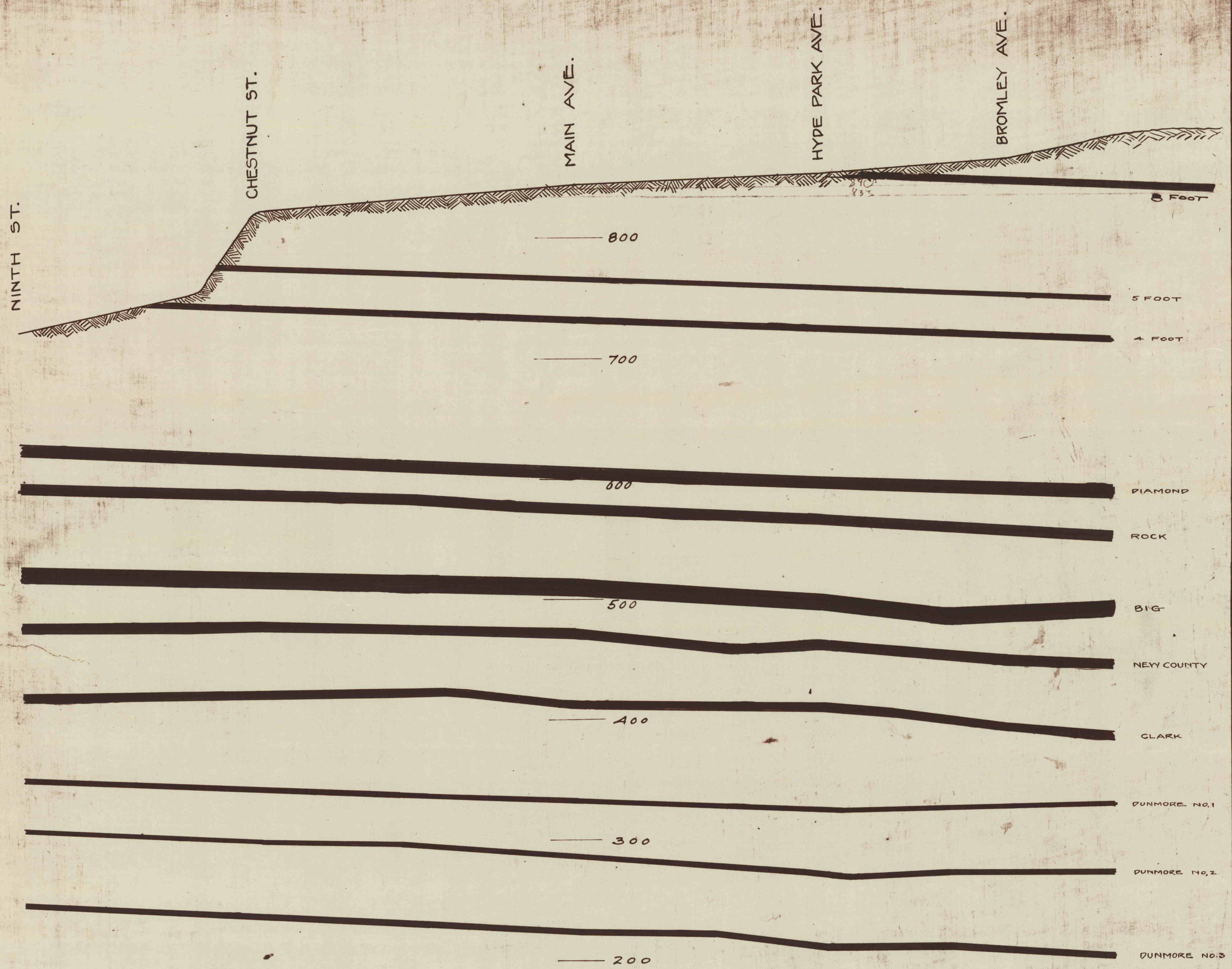
APPROXIMATE CROSS SECTION ALONG LINE OF JACKSON STREET ACROSS PROPERTY OF PEOPLES COAL CO. ~ OXFORD MINES SCRANTON PA.
