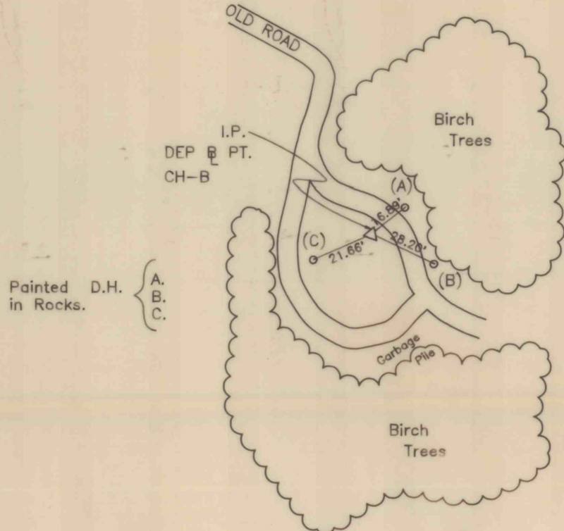
SURVEY REFERENCE CH-B (Not To Scale)
