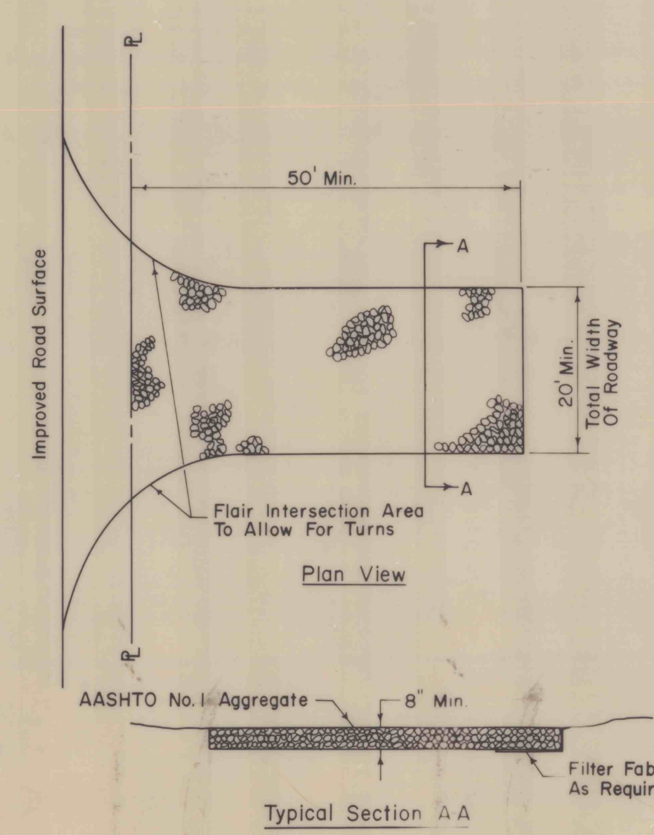
DETAIL ROCK CONSTRUCTION ENTRANCE
