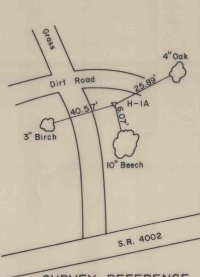
SURVEY REFERENCE
