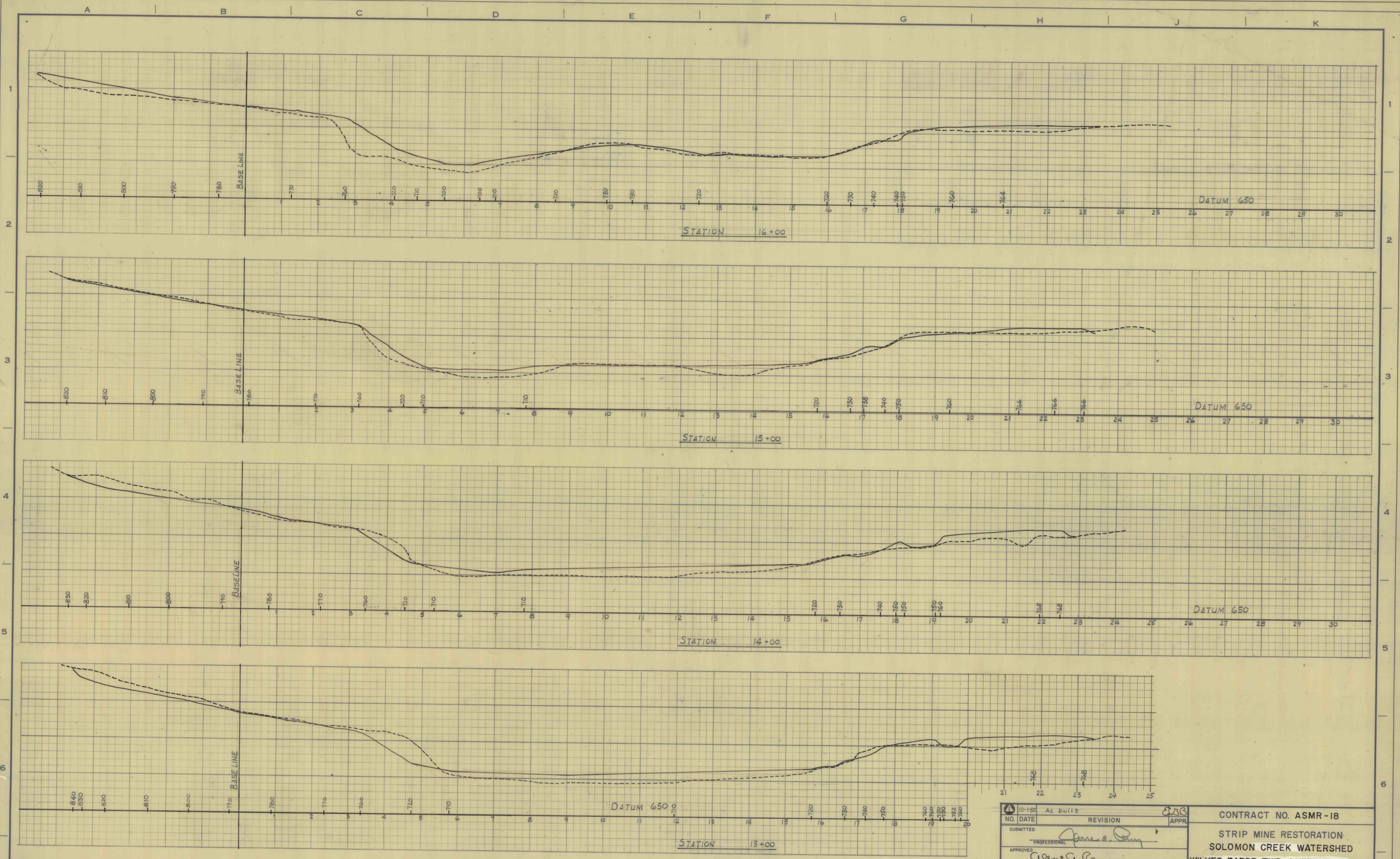
CROSS SECTIONS STATIONS 13+00 THROUGH 16+00 SCALE — HORIZONTAL 1" = 100' VERTICAL 1" = 50'
