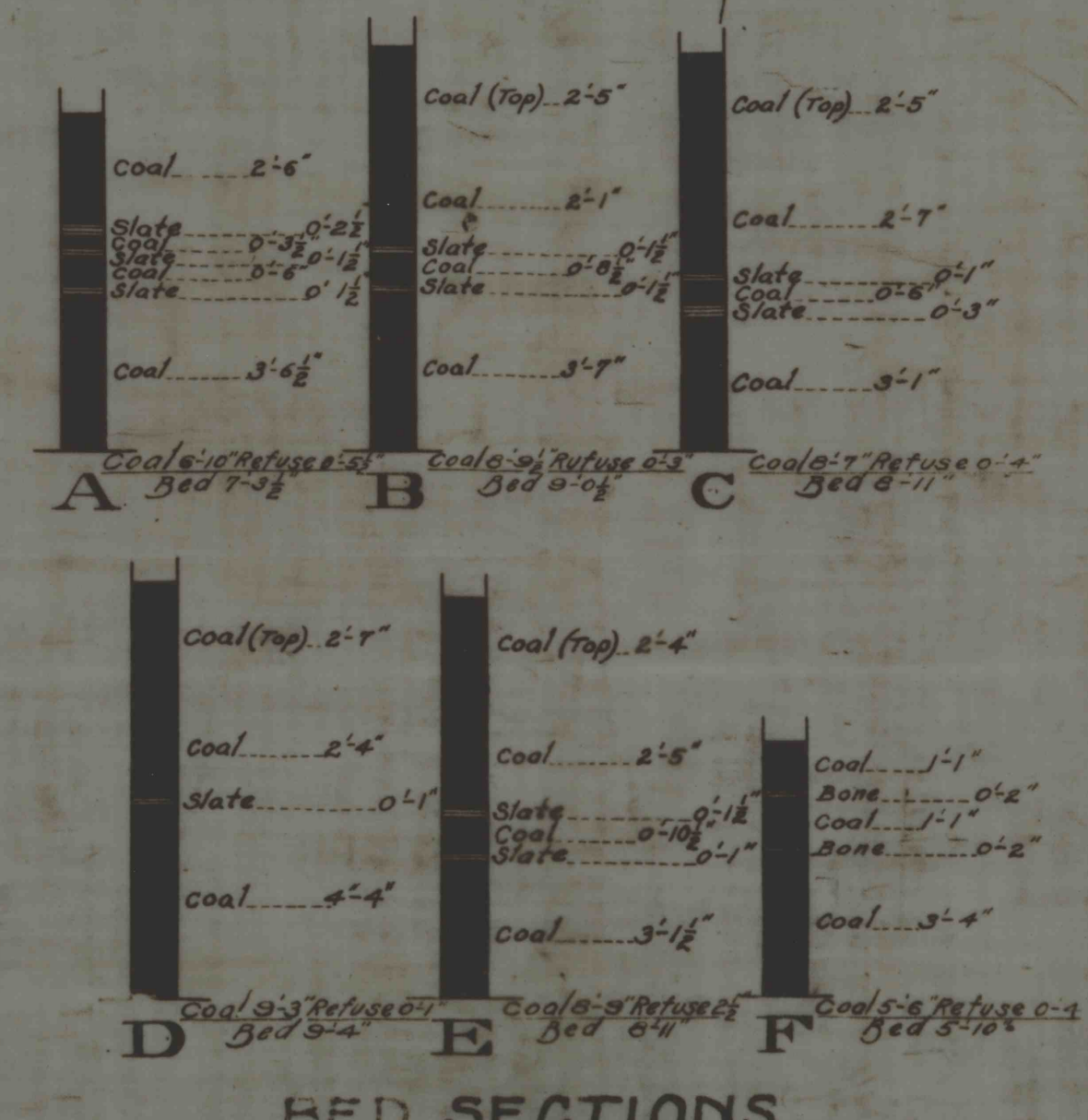
BED SECTIONS
