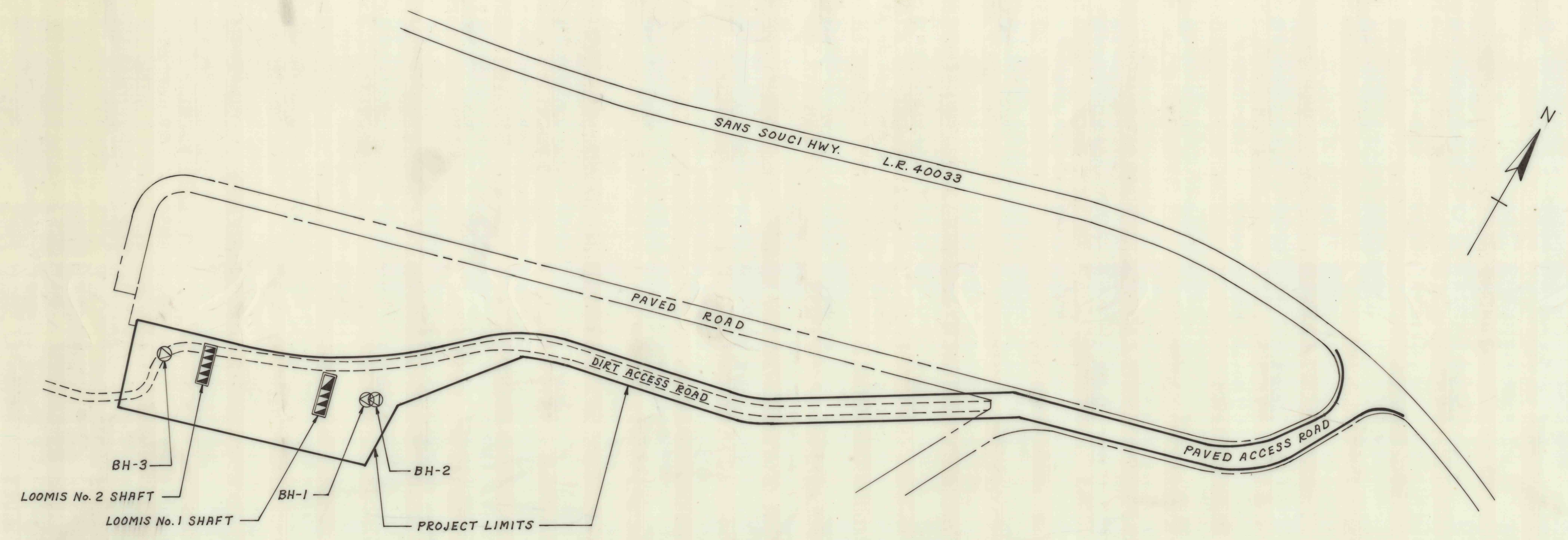
SITE PLAN ANGULAR BORING LOCATIONS
