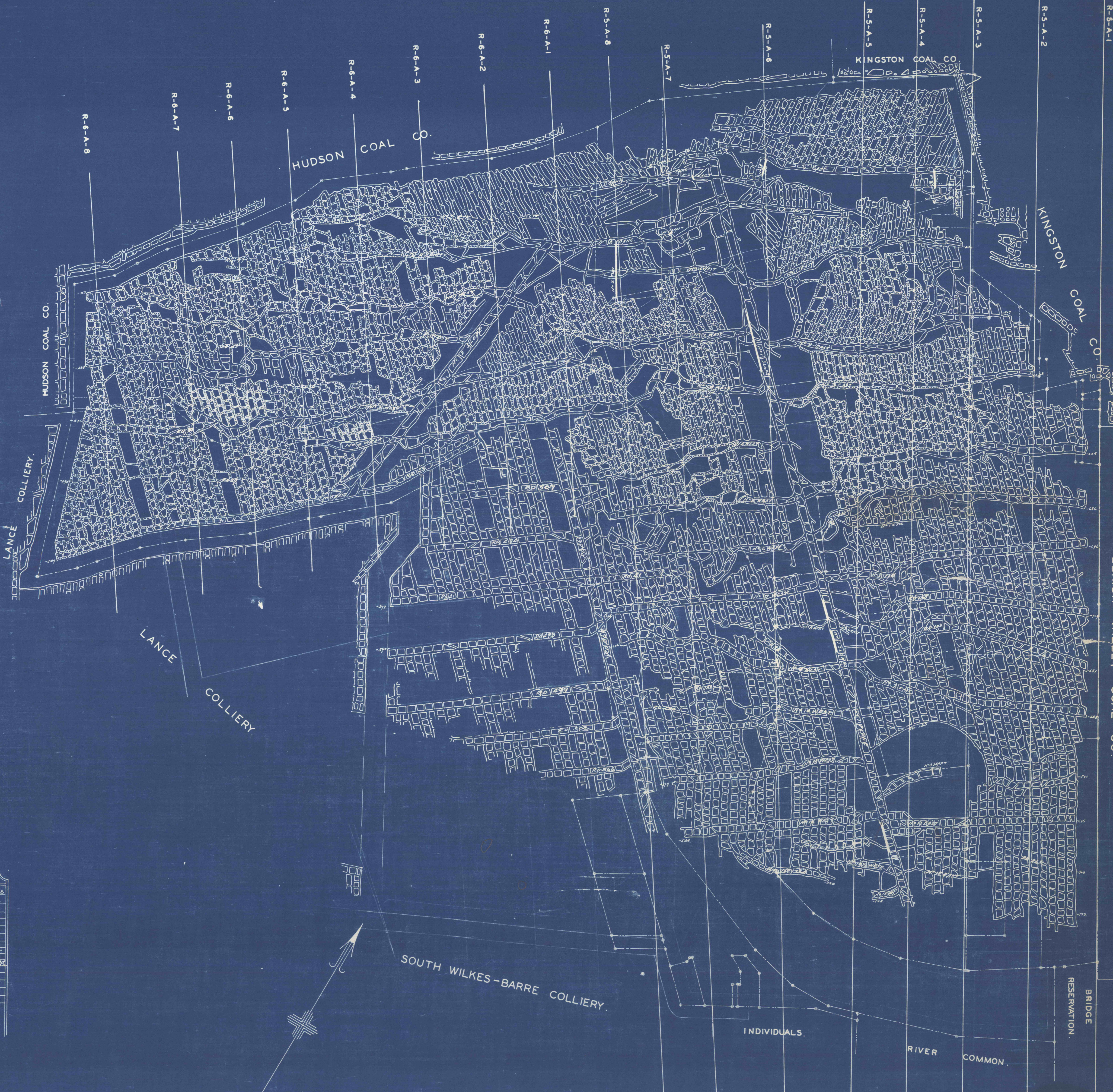
WOODWARD COLLIERY BOTTOM RED ASH VEIN SCALE, 1 INCH = 400 FEET.
