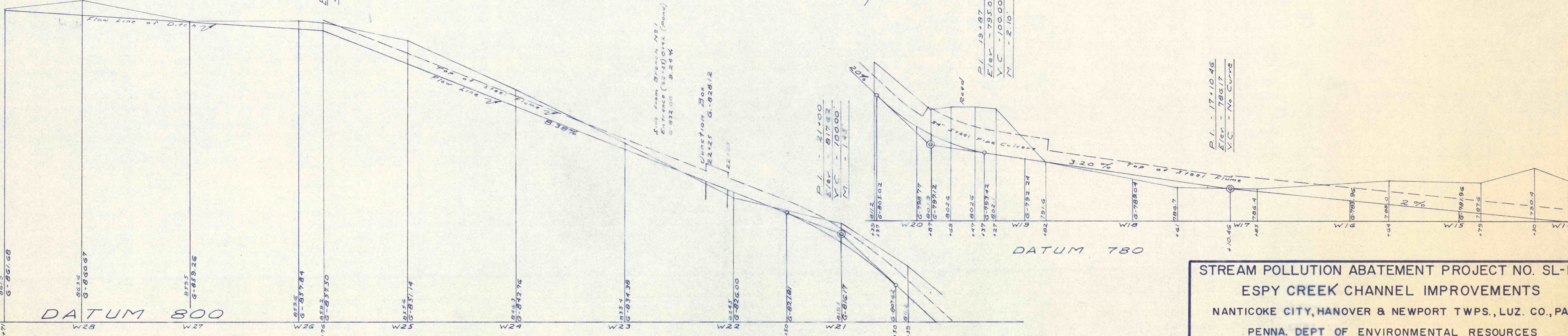
WEST BRANCH - SCALE: HOR. 1"=50' VERT 1"=10'
