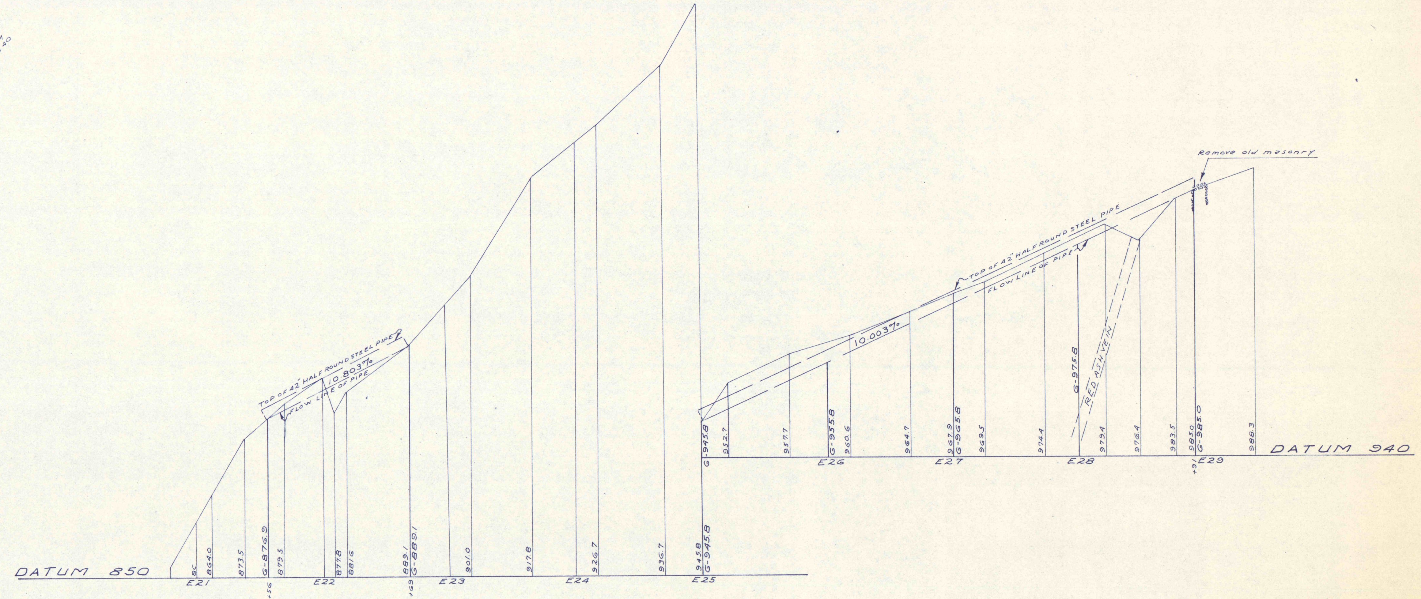
EAST BRANCH PROFILE ALONG \phi OF 42" HALF ROUND STEEL PIPE-LOOKING EAST. SCALE: HORI: 50' VERT. 1" = 10'
