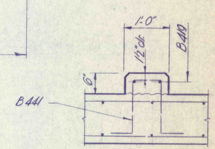
SECT. "B-B" Scale: 3/4" = 1'-0"
