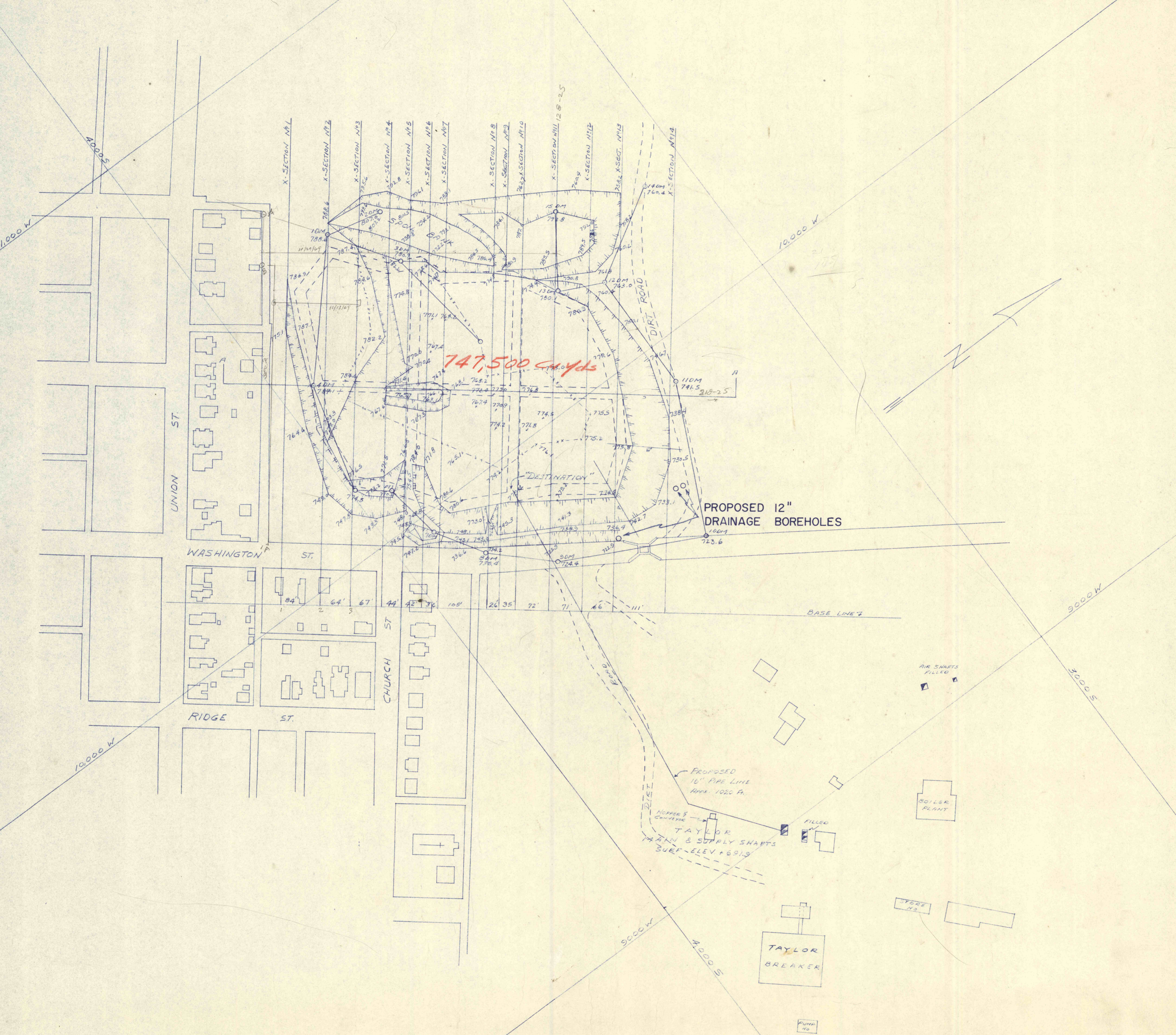
—EXHIBIT A— "THE LAND AND WATER CONSERVATION AND RECLAMATION ACT" AIR POLLUTION ELIMINATION PROJECT NO. SL-203 SURFACE MAP SHOWING BURNING REFUSE BANK UNION AND WASHINGTON STREETS TAYLOR BOROUGH LACKAWANNA COUNTY PENNSYLVANIA DEPARTMENT OF MINES & MINERAL INDUSTRIES SCALE 1" = 100' SEPTEMBER 1968
